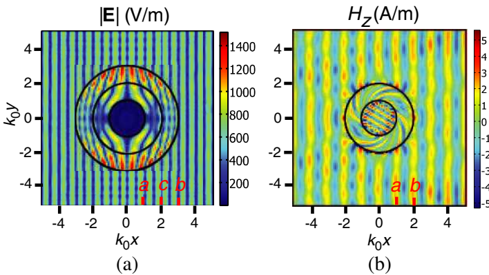
Figure 2. (a) Electric field |\bar{E}| in the two-shell cloak. Plane waves from the left and from the right form the incident standing wave. (b) Magnetic field H_z for the concentrator-rotator application ( A = 3 , \varphi_0 = \pi/3 ). Incident plane wave goes from left to right.
