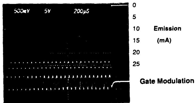
Figure 13. Oscillographs of cathode 100L-A5-1A at 25 mA emission ( 1000 \text{ A/cm}^2 ) with a 6 V peak-to-peak modulation voltage on the gate electrode. Load resistor = 100 \Omega . Anode voltage = 600 V.
