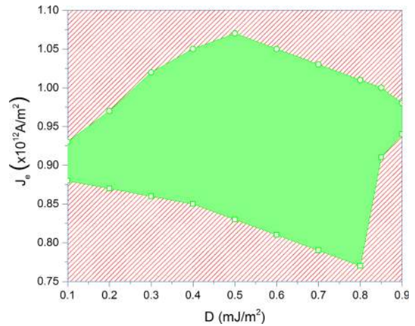
FIG. 5. Deterministic field-free spin-orbit torque switching window for varying DMI constants ( D ) and varying current densities ( J_e ) for a circular device of 100 \text{ nm} diameter. The green region indicates where successful deterministic switching is observed.
