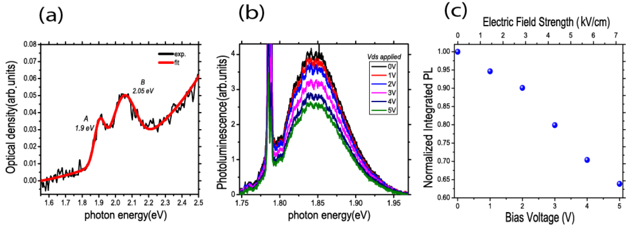
Figure 2. (a) Extinction spectrum of the \text{MoS}_2 monolayer (black curve). Fit by using two Gaussian peaks and a generic exponential function to account for the background from various scattering mechanisms. (b) PL spectra for different bias voltages applied. The feature at 1.78 eV comes from the incomplete subtraction of the sapphire substrate fluorescence (c) Normalized integrated PL as a function of the electric field strength.
