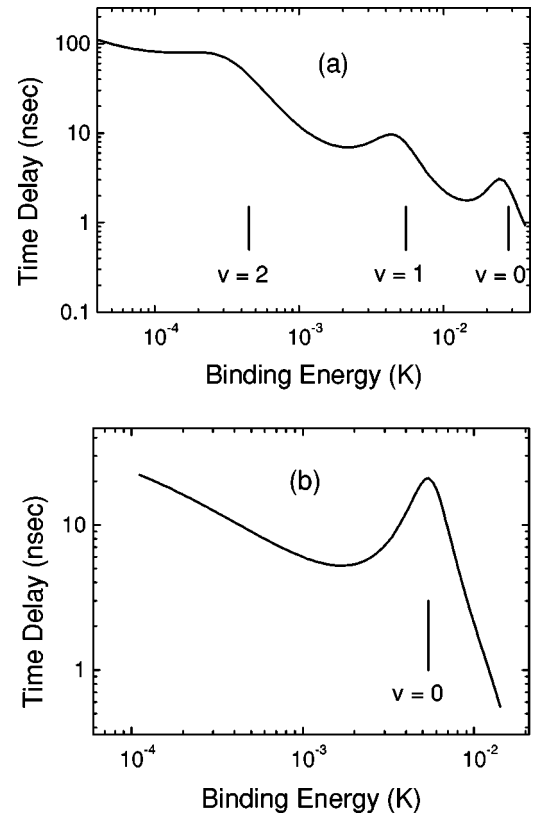
FIG. 5. Time delay as defined in Eq. (20) for the \mathcal{M}=0 (a) and \mathcal{M}=1 (b) FL states. Resonance peaks appear at characteristic energies that correlate well with the binding energies as determined from the FL adiabatic surfaces (vertical lines). Note that the off-resonant time delay can be negative; we have therefore added 6 ns to the computed result, to allow plotting on a logarithmic scale.
