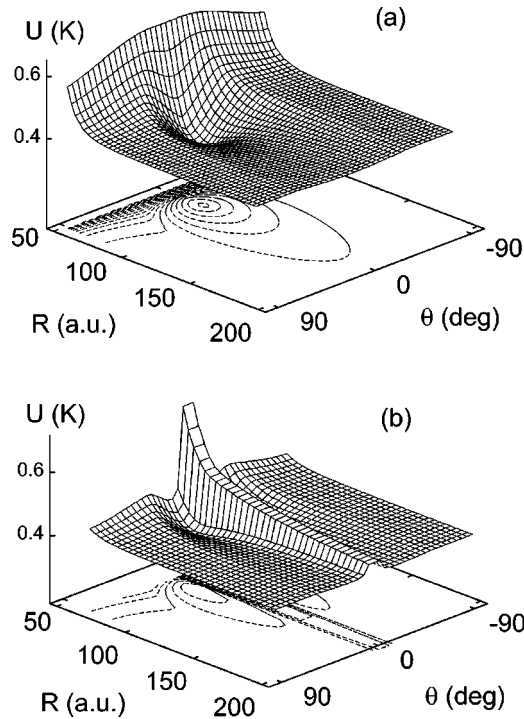
FIG. 2. Adiabatic potential-energy surfaces corresponding to the highest-lying slice in Fig. 1. The M=0 (a) and M=1 (b) cases are shown.
