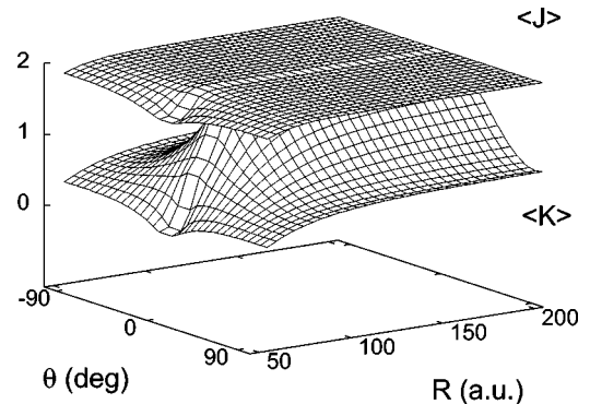
FIG. 3. Average values of J and K for the M=0 potential in Fig. 2. Note that the orientation of the axes is different from that in Figs. 2 and 4.
