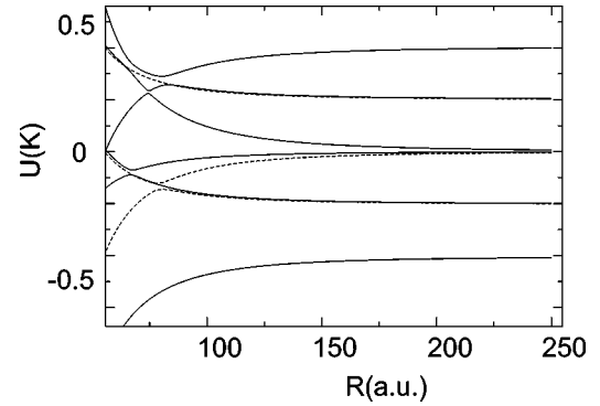
FIG. 1. A “slice” through the adiabatic potential energy surfaces for an electric-field strength \mathcal{E} = 10^4 V/cm. In these surfaces q = -1 , \omega_1 = \omega_2 , and even (solid line) and odd (dashed line) values of \langle J \rangle are distinguished.
