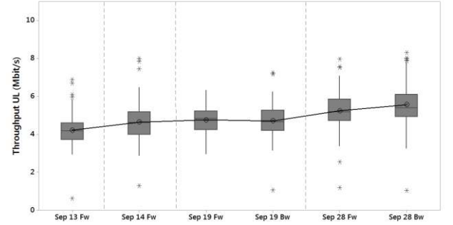
Fig. 10. MP 7 MAC throughput increase during September with H2 configuration.
