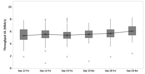
Fig. 9. MP 6 measurements back and forth with H2 configuration.
