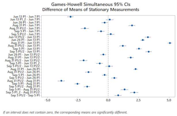
if an interval does not contain zero, the corresponding means are significantly different.
