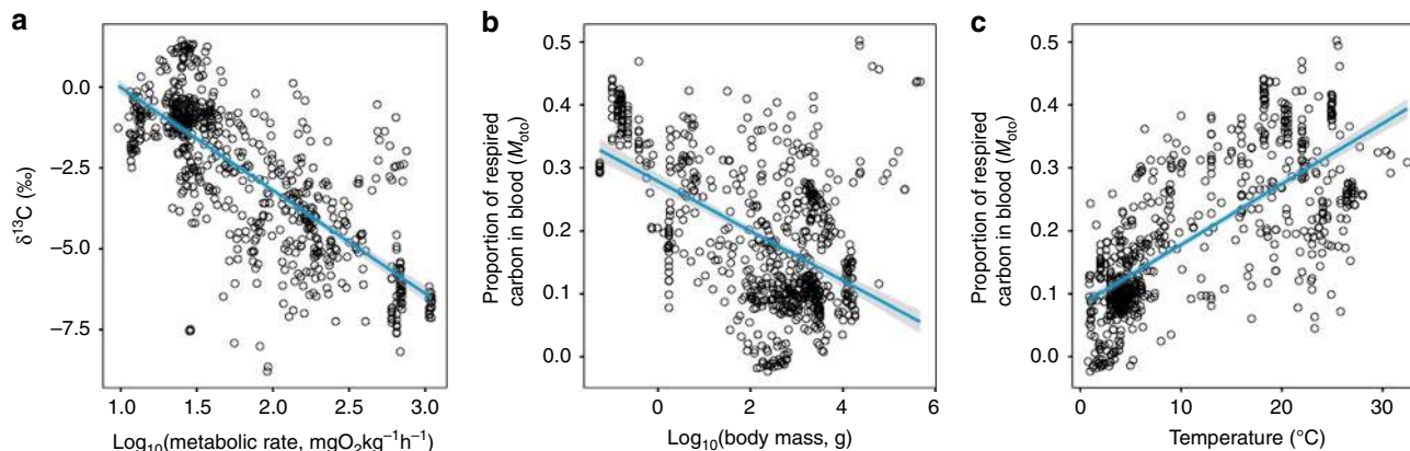
Fig. 2 Among species variations in \delta^{13}\text{C}_{\text{oto}} values and metabolism. a Published \delta^{13}\text{C}_{\text{oto}} values in 76 species covary negatively with estimates of standard metabolic rate predicted by metabolic theory. b The proportion of respired carbon in otolith aragonite ( M_{\text{oto}} ) estimated from \delta^{13}\text{C}_{\text{oto}} values decreases with logarithmic body mass. c M_{\text{oto}} values increase with environmental temperature. (linear regression, temperature: t value = 27.0, p < 0.001 , R^2 = 0.512 ; logarithmic body mass: t value = -16.0, p < 0.001 , R^2 = 0.267 )
