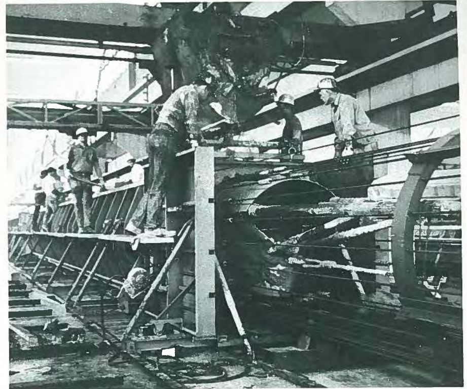
Fig. 83. Formwork and reinforcing cage for casting pretensioned cylinder piles.
