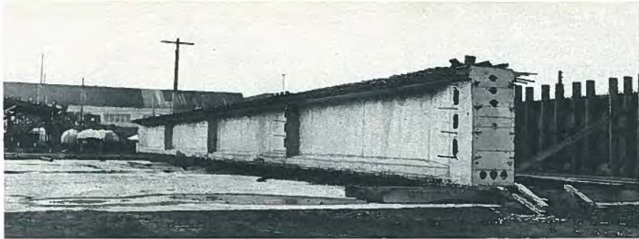
Fig. 77. Completed girder after stripping side forms.
