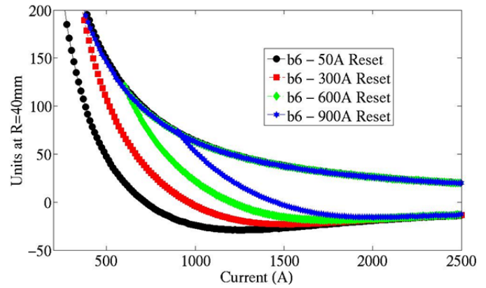
Fig. 9. b_6 during cycles from different minimum currents during accelerator cycles. The value of b_6 at injection can be tuned by choosing the min. current.
