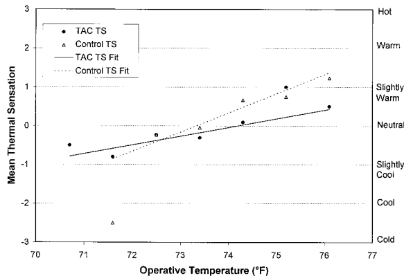
Figure 9b Mean binned thermal sensation votes: TAC group vs. control group, all buildings, July 1996 (I-P).
