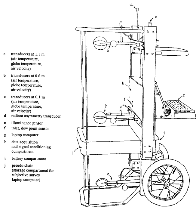
Figure 3 Portable measurement cart.
