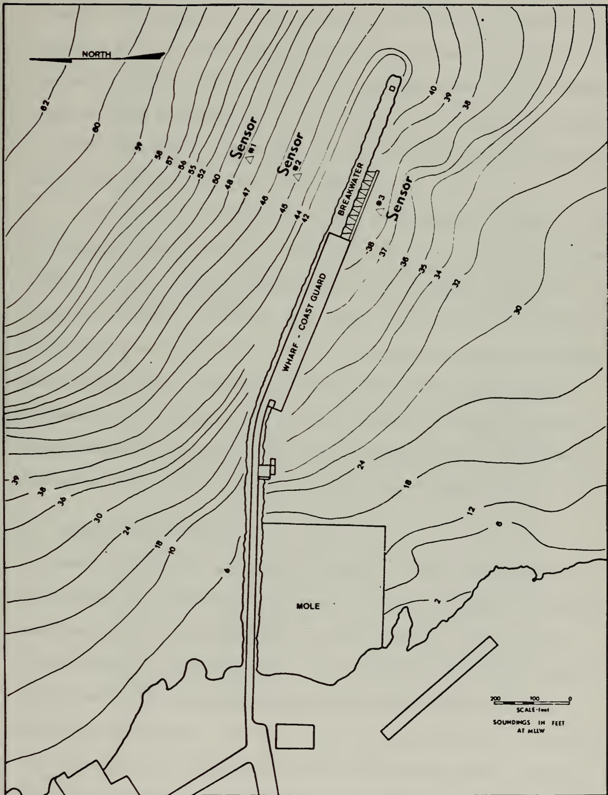
FIGURE 4 Monterey Breakwater
