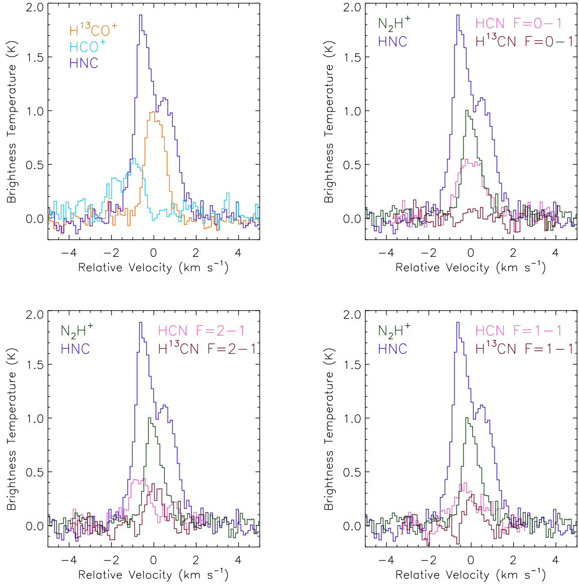
Figure 7. A comparison of the self-absorption profiles for HCO + , and the three hyperfine components of HCN. The HNC emission is shown in dark blue, while H 13 CO + is in orange, the isolated hyperfine component of N 2 H + (F 1 , F=0,1-1,2) is in green, HCO + is shown in light blue, and each component of HCN / H 13 CN is shown in light / dark pink. In the case of lines with hyperfine components, the velocity centroid has been shifted to the appropriate common centre. Note that no scaling has been applied to the brightness temperatures shown.
