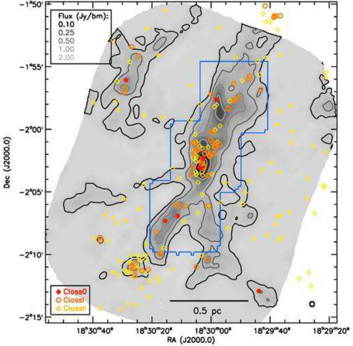
Figure 1. The large-scale context of our Mopra observations of Serpens South. The greyscale image and contours show an AzTEC/ASTE map of the millimetre dust continuum emission, while the red filled circles, orange open circles, and yellow diamonds show the YSO population found in Spitzer data. The black circle at the bottom right corner shows the AzTEC/ASTE beamsize (28'' FWHM). The blue contour shows the region mapped with Mopra, covering all of the main filamentary structure.
