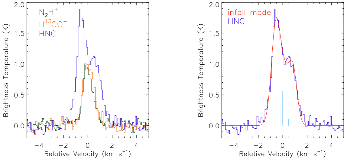
Figure 6. Left: the N 2 H + (green) and H 13 CO + (yellow), and HNC (blue) average spectra for the southern filament. (For N 2 H + , only the isolated hyperfine component, (F 1 ,F=0,1-1,2), is shown.) The HNC spectrum shows clear signs of self-absorption, while the N 2 H + and H 13 CO + spectra are well described by a single Gaussian. Right: The filament-averaged HNC profile, along with the expected relative positions and strengths of the hyperfine emission lines of HNC. The hyperfine splitting is on too small a scale to be responsible for the observed self-absorption profile. The red line shows the best fit Hill5 infall model profile (deVries & Myers 2005). See text for details.
