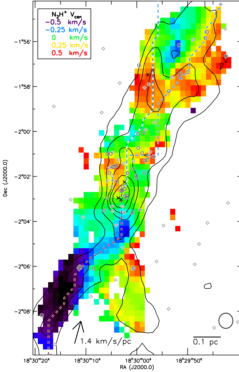
Figure 4. The centroid velocity measured for \text{N}_2\text{H}^+ across Serpens South. The contours correspond to the dust emission levels shown in Figure 1 and 3, and the circles denote the same YSOs as shown in Figure 1 (dark grey corresponds to class 0, medium grey to class I and light grey to class II sources). The peak ridge of the filament is shown by the dashed lines (red in the south and blue in the north for clarity). The overall velocity gradient measured in the southern filament is indicated by the arrow at the bottom left, while the circle at the bottom right indicates the Mopra beamsize.
