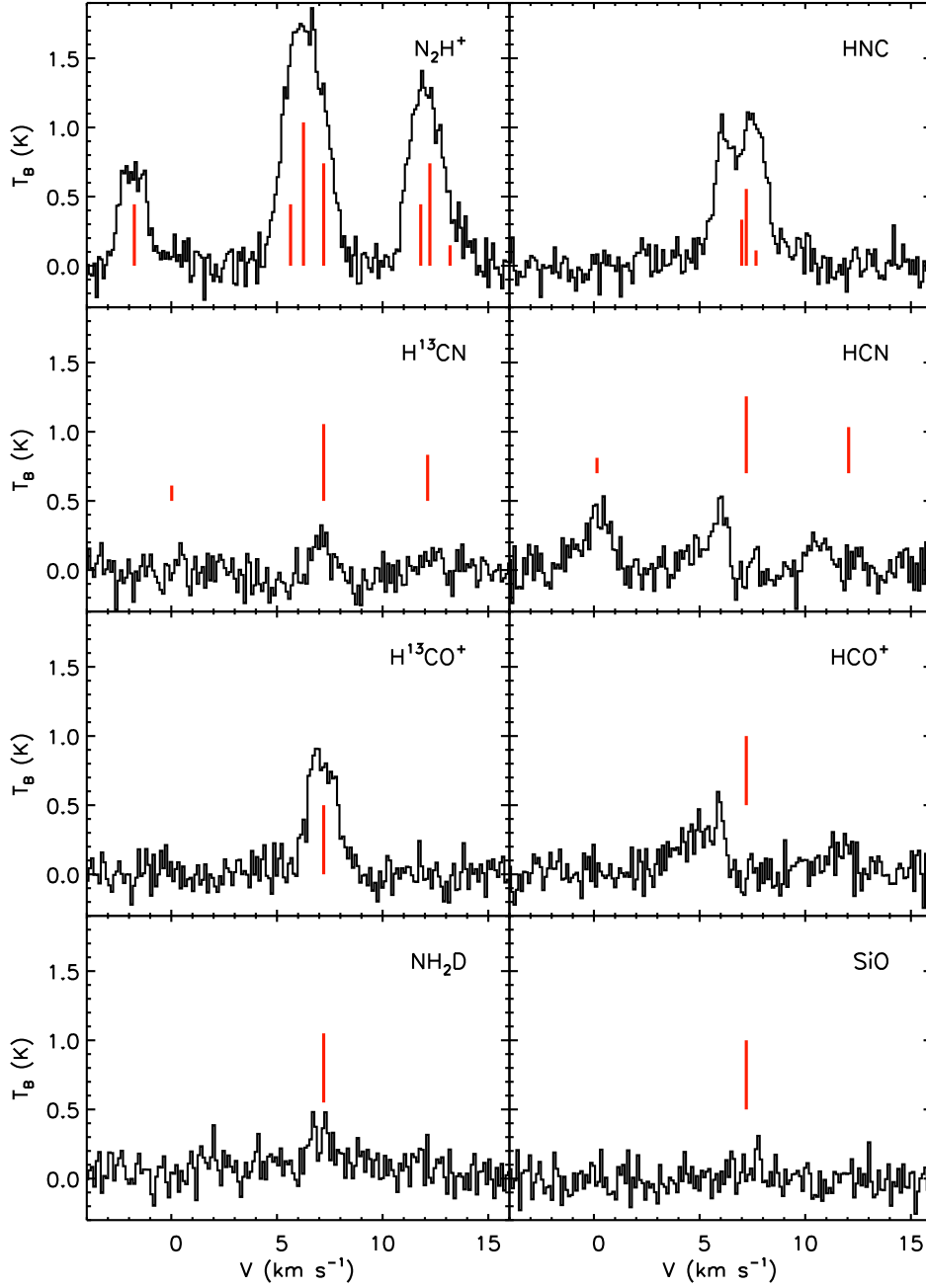
Figure 2. The observed emission lines near the cluster centre ( -18^h30^m01^s, -2^{\circ}03'12'' ). The data have been summed over 4 \times 4 pixels (an area of 60 by 60'' ) to increase the signal to noise level. The red vertical lines indicate the expected line centres based on a fit to the \text{N}_2\text{H}^+ spectrum. In the case of (discernable) hyperfine components, all are shown, with the relative heights scaling with the optically thin line ratios. Note that \text{SiO} emission was not detected with certainty anywhere in the map.
