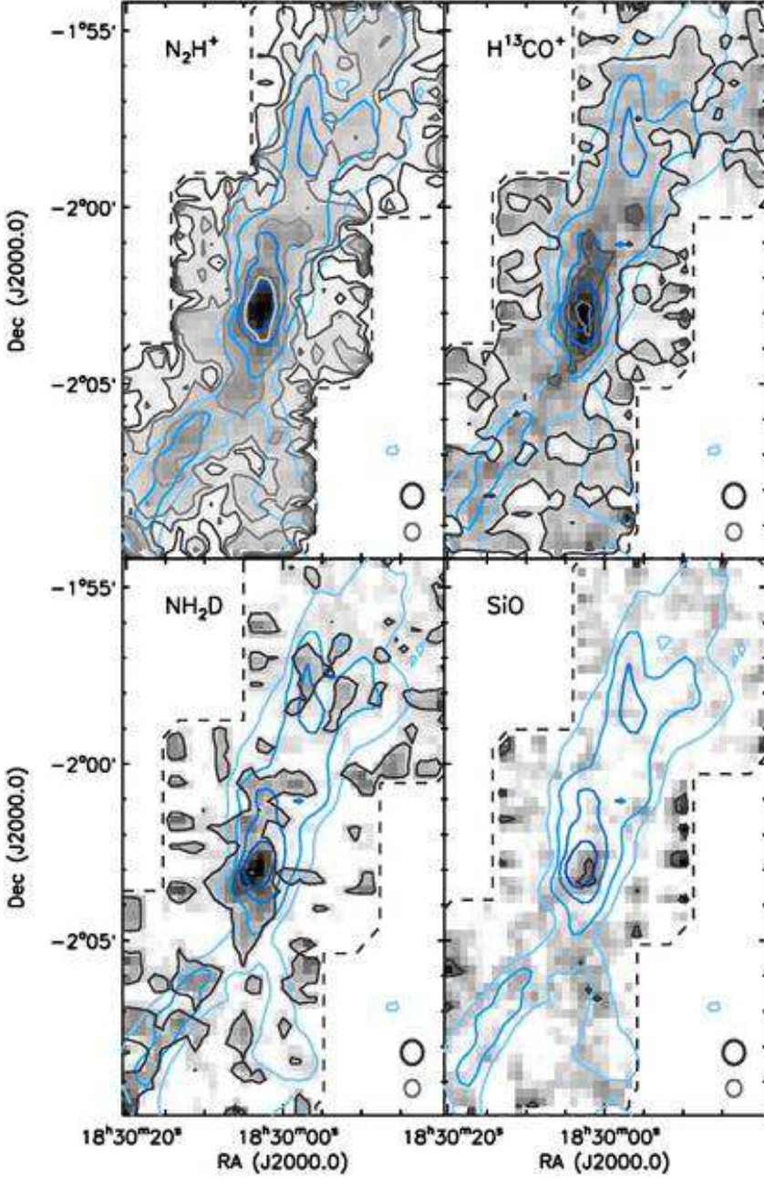
Figure 3. The integrated intensity of the three brightest molecular tracers in our survey not affected by self-absorption ( \text{N}_2\text{H}^+ , \text{H}^{13}\text{CO}^+ , \text{NH}_2\text{D} ), as well as \text{SiO} , which should not show self-absorption, but has no clearly detected emission. The greyscale images show the integrated intensities, with white at a value of -0.1 \text{ K km s}^{-1} and black at a value of 90% of the maximum integrated intensities measured in each molecular species (23.5, 3.8, 3.2, and 1.2 \text{ K km s}^{-1} respectively). The grey contours in all panels are at values of 0.5, 2, 3.5, 7, and 15 \text{ K km s}^{-1} from darkest to lightest. The dashed line indicates the full region mapped by Mopra, and the blue contours show the dust emission from AzTEC/ASTE, at levels of 0.25, 0.5, 1, and 2 \text{ Jy bm}^{-1} from light to dark. The Mopra and AzTEC/ASTE beams are shown on the bottom right of each panel in dark and light grey respectively.
