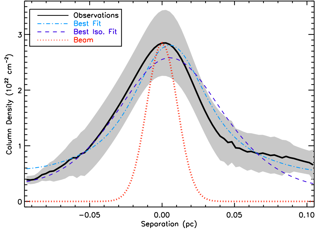
Figure 8. The radial column density profile of the southern filament in Serpens South. The solid black line shows the mean profile across the filament, while the grey shaded area indicates the standard deviation. The AzTEC/ASTE beamsize is shown by the red dotted line. The light blue dash-dotted line shows the best fit profile, following the formulation in Arzoumanian et al (2011), while the dark blue dashed line indicates the best fit profile when the power law index is that corresponding to an isothermal cylinder.
