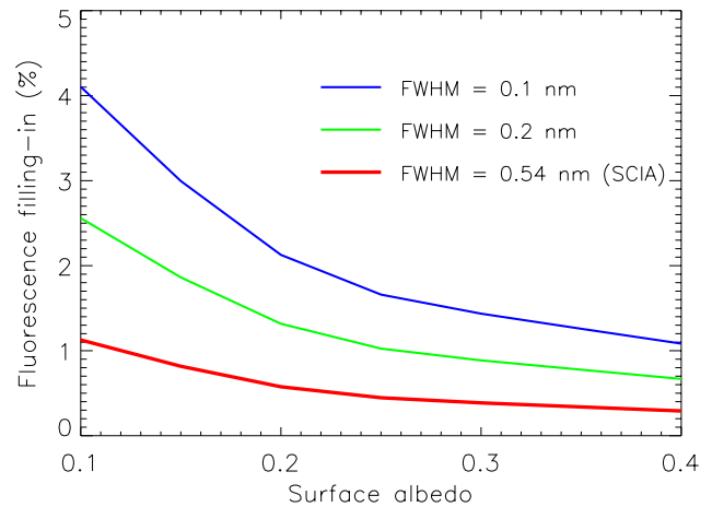
Fig. 3. Filling-in due to an additive signal of 0.2 \text{ mW m}^{-2} \text{ nm}^{-1} \text{ sr}^{-1} , \text{SZ} = 20^\circ , and nadir as a function of surface reflectivity for different instrument spectral resolutions.
