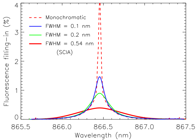
Fig. 2. Simulated spectral filling-in around the Ca II solar line from an additive signal of 0.2 \text{ mW m}^{-2} \text{ nm}^{-1} \text{ sr}^{-1} , \text{SZ} = 40^\circ nadir, and surface reflectivity = 0.3 (RRS not included) for different instrument resolutions (triangular slit function) with full-width half-maximum (FWHM) as indicated including that of SCIAMACHY (SCIA).
