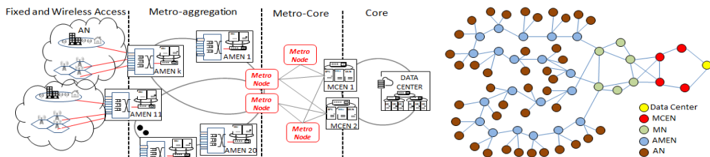
Figure 2 A schematic representation of the network topology showing the 4 network levels (left) and the network topology considered in our study (right).
