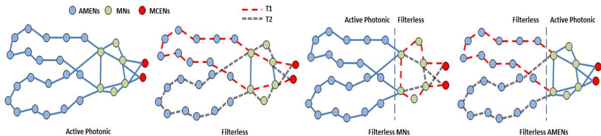
Figure 3 (From left to right) The network topology for the Active Photonic and the fiber tree formation for the Filterless , the Filterless MN and the Filterless AMENs . Note that the ANs are not sketched as they act as leaves and belong to the same fiber.
