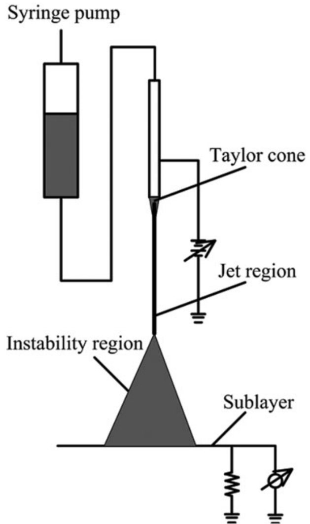
Figure 1 Experiment set-up.
