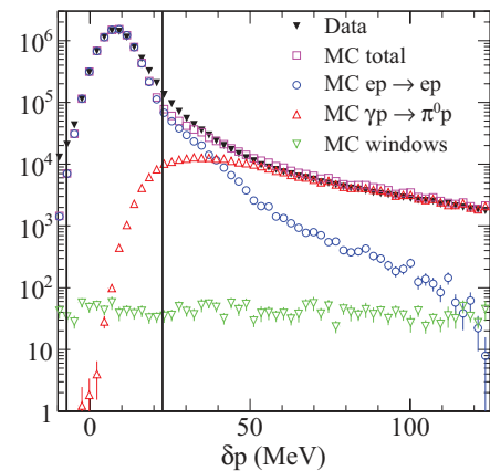
FIG. 10. (Color online) Contributions to the \delta p distribution at Q^2 = 4.8 \text{ GeV}^2 estimated from the Monte Carlo simulation. Monte Carlo distributions are shown for elastic ep \rightarrow ep (open circles), \gamma p \rightarrow \pi^0 p (open triangles), and quasielastic ( e, e'p ) in the target windows (open inverted triangles). The sum of all Monte Carlo contributions (open squares) is compared to the data of Fig. 5(c) (solid inverted triangles). Monte Carlo and data distributions are obtained after applying \Delta x and \Delta y (calorimeter) cuts. Black vertical lines show the \delta p cut region of the final analysis. Uncertainties shown are statistical only. See text for details.
