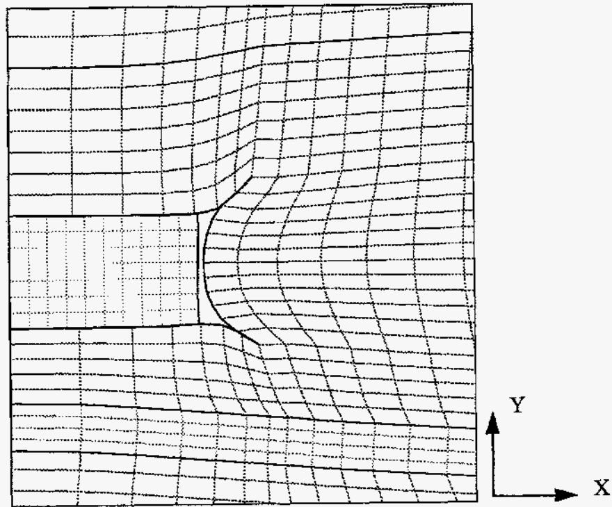
Figure 11. Close-up View of the Deformed Disposal Room With Waste at 300 Years for f = 0.5 .
