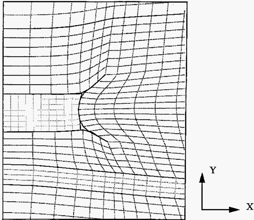
Figure 9. Close-up View of the Deformed Disposal Room With Waste at 300 Years for f = 0.0 .
