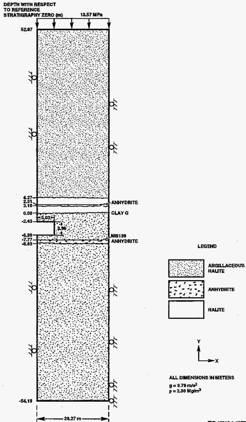
Figure 4. Simplified Stratigraphic Model Used For the Current Disposal Room Analyses (Butcher, 1997).
