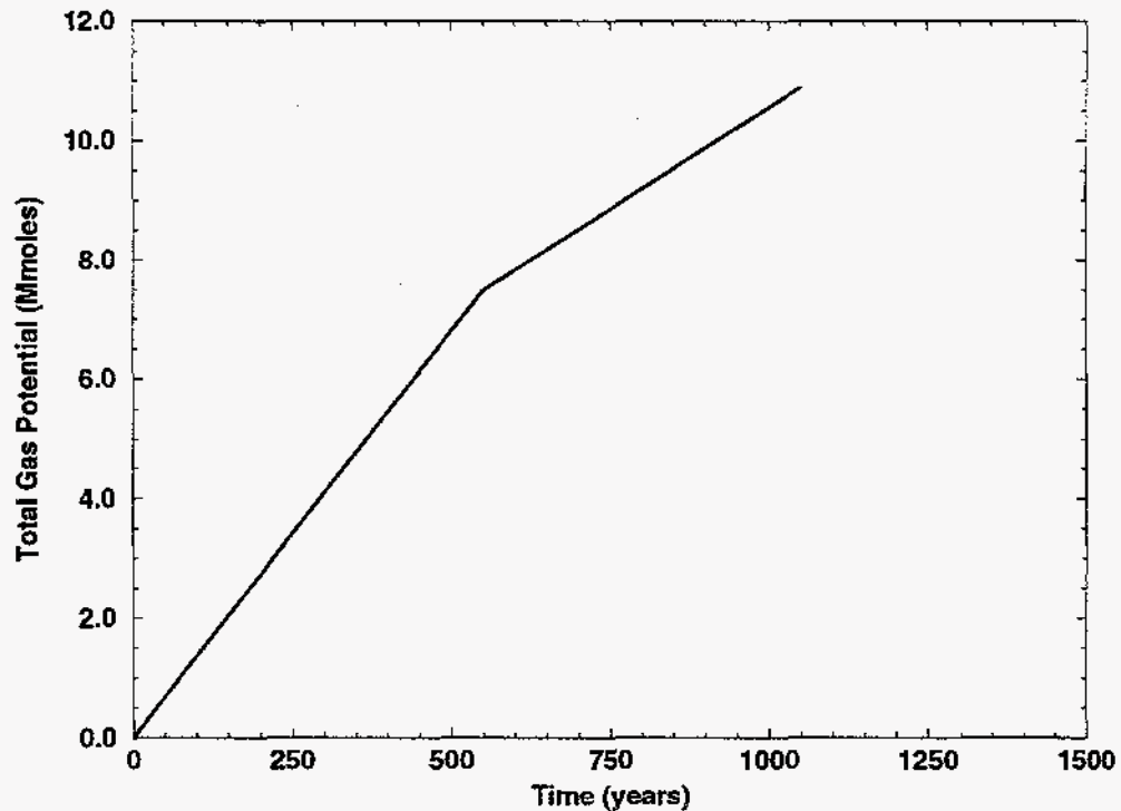
Figure 2. History of the Reference Gas Generation Potential Used for the Disposal Room Analyses, f = 1.0 .
