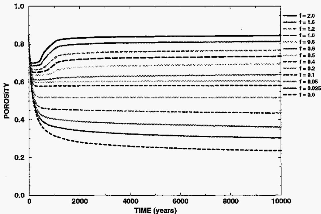
Figure 8. Porosity Histories for Various Values of the Gas Generation Parameter, f , for a Disposal Room Containing Waste Only. The Gas Generation Parameter Values Range From Bottom to Top: f = 0.0, 0.025, 0.05, 0.10, 0.20, 0.40, 0.50, 0.60, 0.80, 1.0, 1.2, 1.6, and 2.0 .
