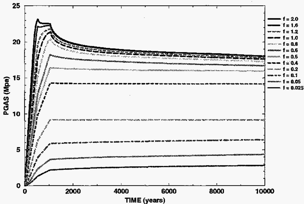
Figure 7. Pressure Histories for Various Values of the Gas Generation Parameter, f , for a Disposal Room Containing Waste Only. The Gas Generation Parameter Values Range From Bottom to Top: f = 0.025, 0.05, 0.10, 0.20, 0.40, 0.50, 0.60, 0.80, 1.0, 1.2, 1.6, and 2.0 .
