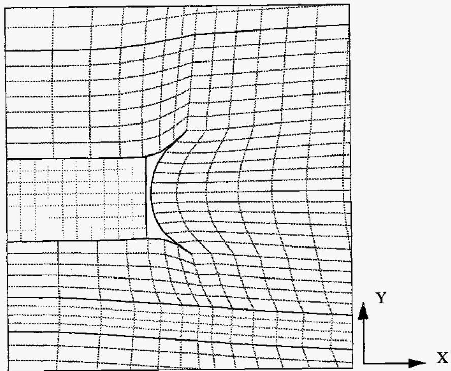
Figure 12. Close-up View of the Deformed Disposal Room With Waste at 10,000 Years for f = 0.5 .
