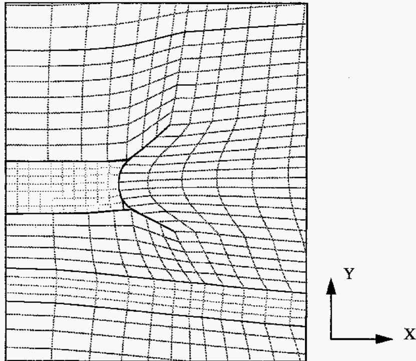
Figure 10. Close-up View of the Deformed Disposal Room With Waste at 10,000 Years for f = 0.0 .
