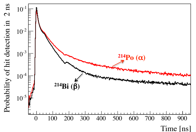
FIG. 27. The reference r_\alpha(t_n) (red) and r_\beta(t_n) (black) pulse shapes obtained by tagging the radon-correlated ^{214}\text{Bi} - ^{214}\text{Po} coincidences. The dip at 180 ns is due to the dead time on every individual electronic channel applied after each detected hit (see Section VI). The small shoulder around 60 ns is due to the light reflected on the SSS surface and on the PMTs' cathodes.
