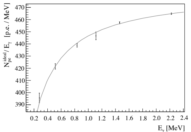
FIG. 46. Data points for six different \gamma -ray lines: ^{203}\text{Hg} , ^{85}\text{Sr} , ^{54}\text{Mn} , ^{65}\text{Zn} , ^{40}\text{K} , and the 2230 keV \gamma from the neutron capture: N_{pe}^{\text{ideal}}/\text{MeV} expressed as a function of E_\gamma . The data is fit with the function corresponding to Eq. 42 which is obtained by a dedicated “ad hoc” Monte Carlo using the Birk’s quenching model (details in text). The best fit values are kB = 0.00115 \pm 0.0007 and Y_0^{pe} = 489 \pm 2 p.e./MeV.
