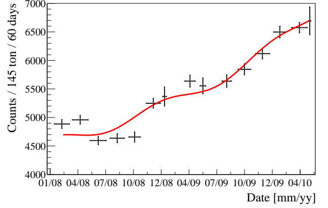
FIG. 63. Results obtained with rate analysis. The continuous line is the curve of Eq. 84. The data are grouped in bins of 60 days.
