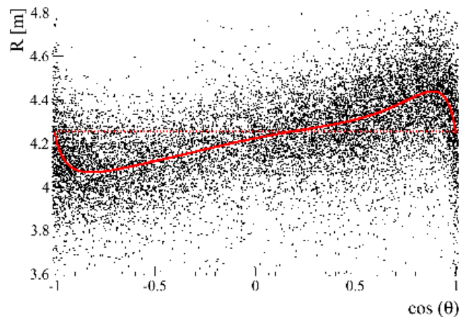
FIG. 19. R - \cos(\theta) distribution of the events in the energy region 800 - 900 keV from November 2007 used for the IV shape reconstruction. The best-fit vessel shape is shown in a solid red line. The dotted red line represents the nominal spherical vessel with R = 4.25 m.
