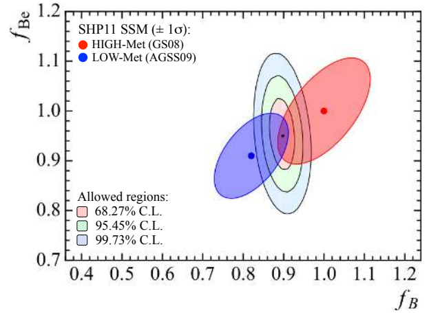
FIG. 82. The 1\sigma theoretical range of high (red) and low (blue) metallicity Standard Solar Model for f_{\text{Be}} and f_{\text{B}} , compared to the 1\sigma (light pink), 2\sigma (light green), and 3\sigma (light blue) allowed regions by the global analysis of solar-with Borexino plus KamLAND results. The theoretical correlation factors are taken from [87].
