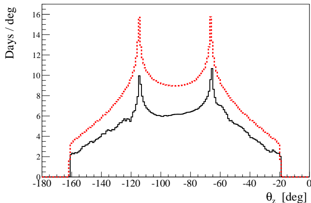
FIG. 56. The experimental exposure function (black continuous line) and the ideal exposure function (red dotted line) corresponding to 3 years of data taking without interruptions at LNGS, as functions of the \theta_z angle (1 deg/bin). The interval from -180^\circ to -90^\circ corresponds to day (360.25 days) and the one from -90^\circ to 0^\circ to night time (380.63 days). We recall that at LNGS latitude the Sun is never at the zenith.
