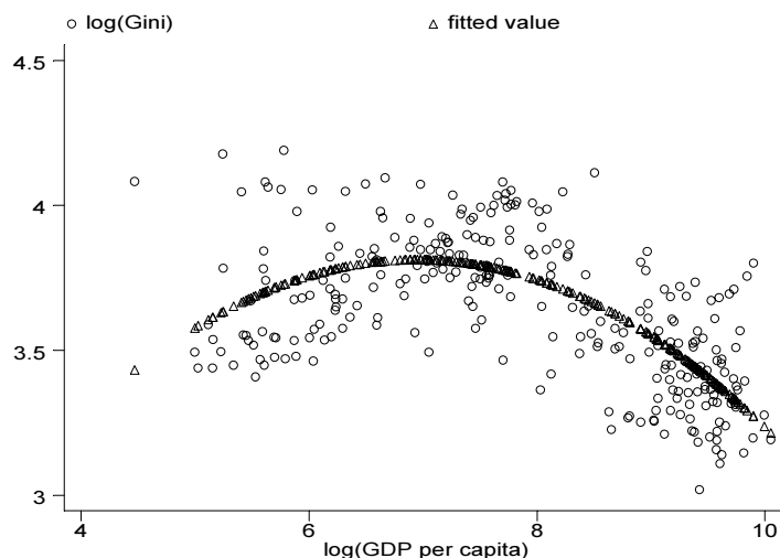
FIG. 1. Log (Gini) and Log(GDP per capita) in a panel of 91 countries
