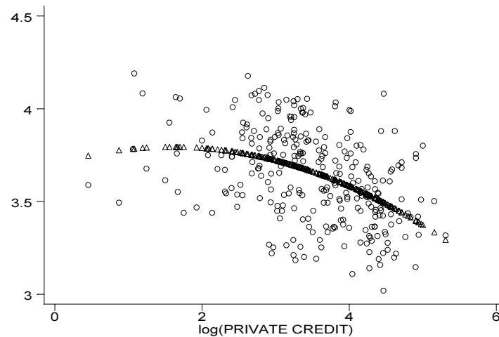
FIG. 2. Log (Gini) against Log (Private Credit) in a panel of 91 countries ○ log(Gini) △ fitted value
