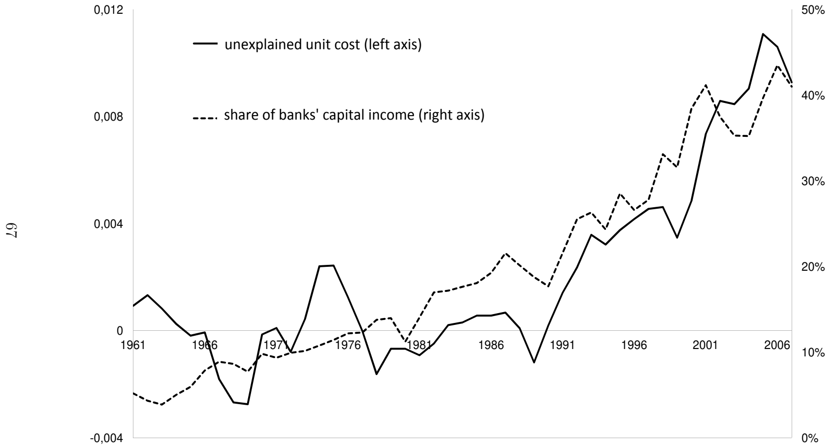
Figure 4.2.1c: unexplained unit cost and banks' share of capital income in Europe
