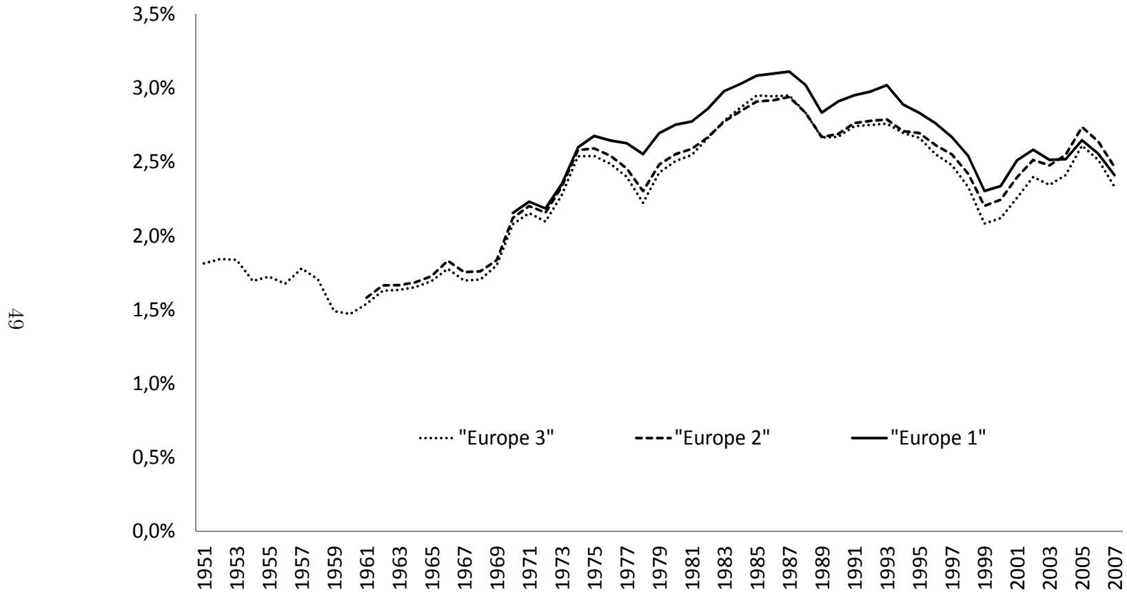
Figure 3.1.3: Unit cost of financial intermediation, European estimation, first method
