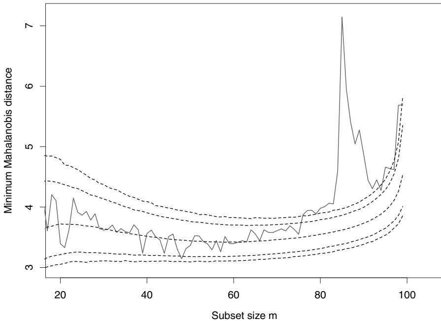
Fig. 1. Swiss banknotes, forgeries ( n = 100 )—forward plot of the minimum unscaled Mahalanobis distance with superimposed 1%, 5%, 95% and 99% bootstrap envelopes from 10000 simulations: there is a clear indication of the presence of outliers which starts around m = 84
