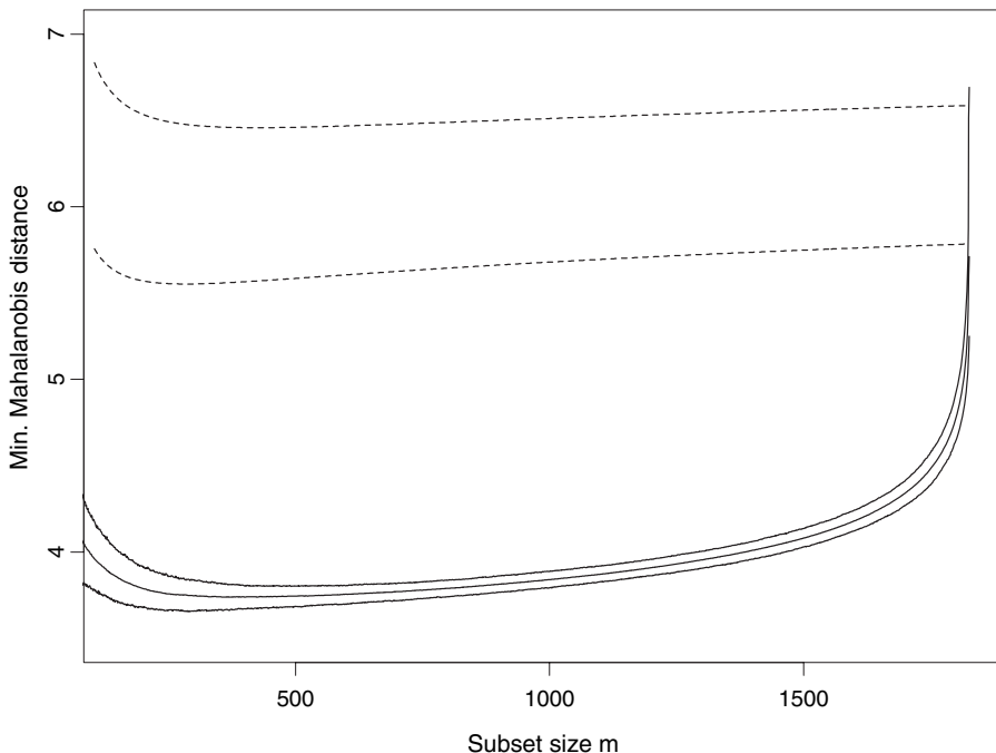
Fig. 3. 2000 normal observations, v = 10 : forward plot of 90% and 99% envelopes of minimum Mahalanobis distances with superimposed Bonferroni bounds including Hadi’s correction
