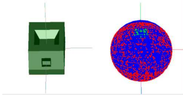
Figure 11: Sample part with castable directions shown by the (lighter) green dots on the Gaussian sphere. Non-castable directions are shown by (darker) red dots.
