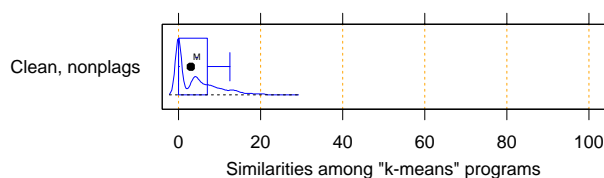
Figure 6: Distribution of similarity values found among all pairs in Clean . This program set does not contain any plagiarisms at all and all program pairs have rather low similarity values. The maximum is 27.
