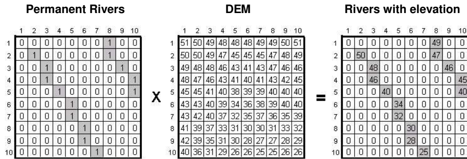
Figure 4.5 Raster Calculation of Permanent Rivers and the DEM in order to receive a layer with Permanent Rivers with height values. Grey cells represent river cells and the values in the DEM represents height values in meters.
