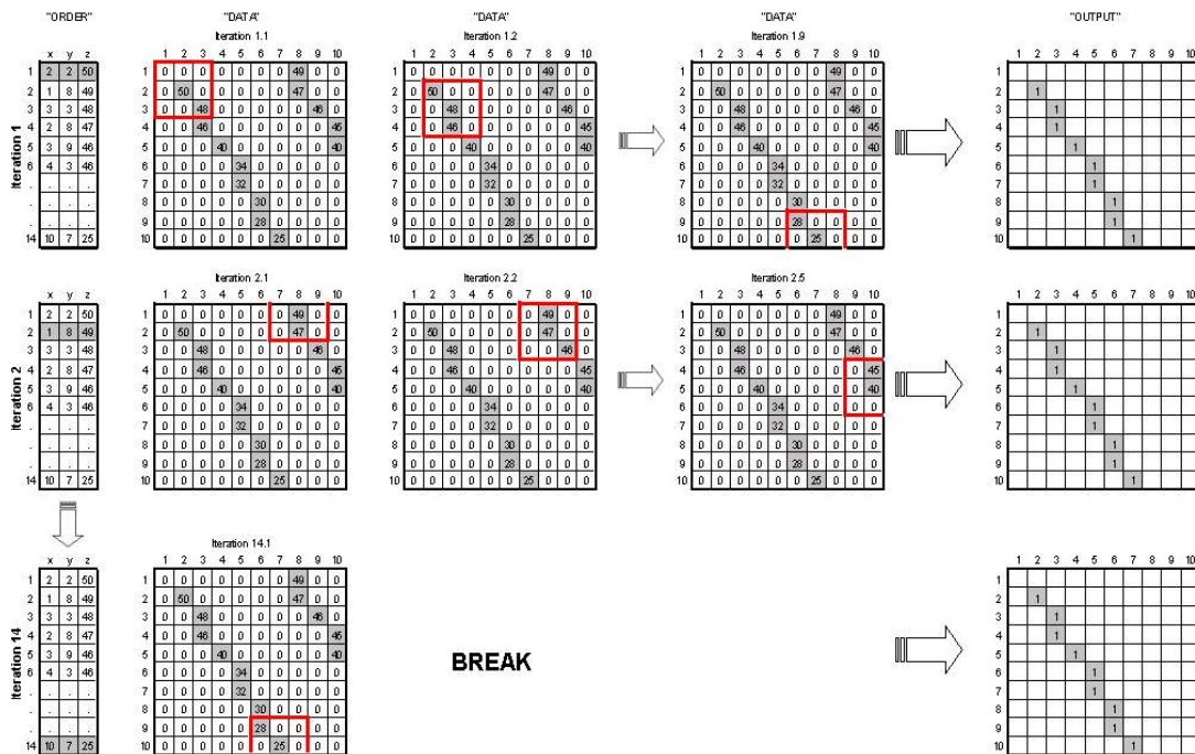
Figure 4.9 An example of how the “3 x 3 search window” operation works in a fictitious raster.
