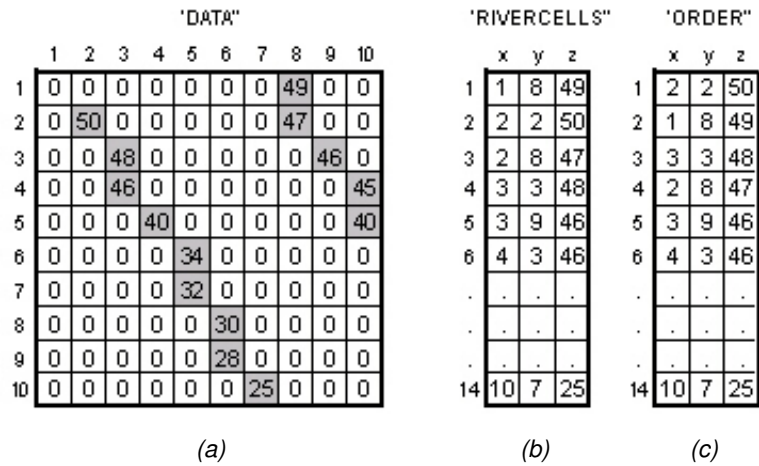
Figure 4.8 An example showing the matrix “DATA” (a) and the arrays “RIVERCELLS” (b) and “ORDER” (c).
