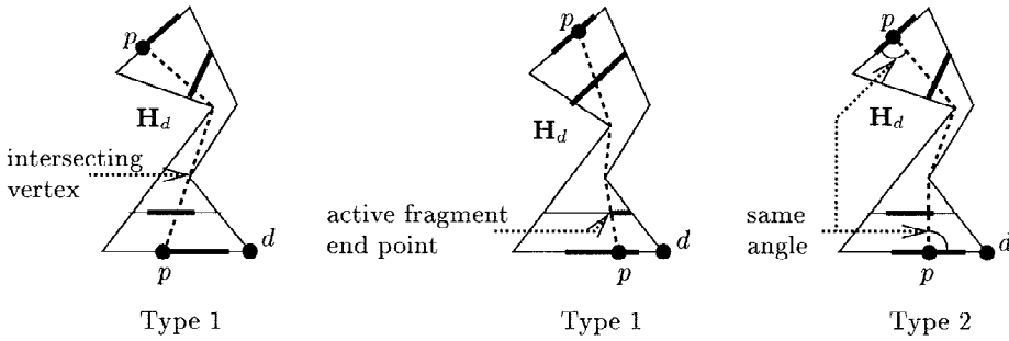
Fig. 7. The event points of the sliding process.
