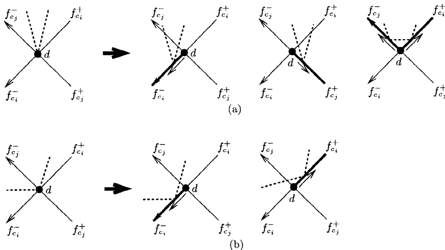
Fig. 11. The different cases of sliding depending on the initial route W_d .
