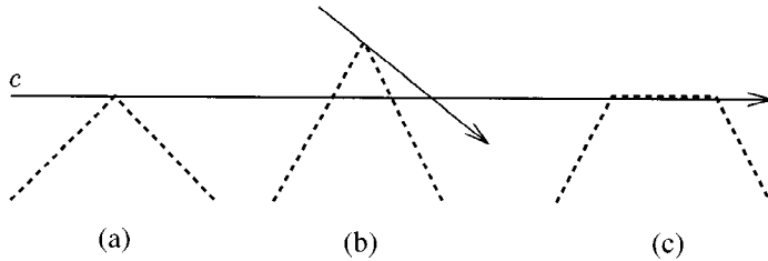
Fig. 3. The three different types of possible contacts made by a shortest watchman route.
