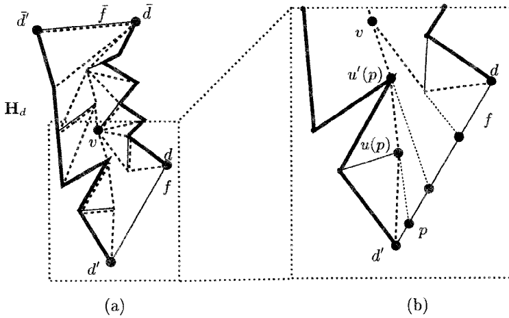
Fig. 12. Illustrating the computation of Type 1 event points from SPT_{\bar{d}} .
