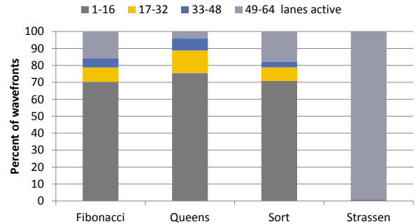
Figure 19: Branch divergence
