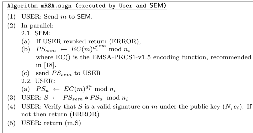
Fig. 2. mRSA Signature Algorithm
