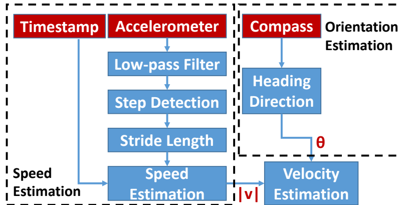
Figure 3: Velocity Estimation
