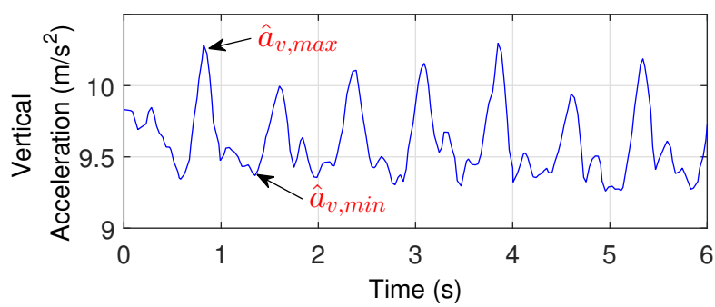
Figure 4: Vertical Acceleration
