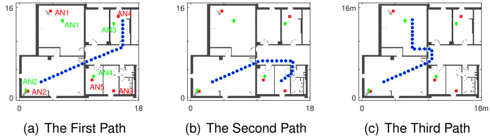
Figure 6: Tracking in Different Paths (Diamond Points: ANs in Scenario 1; Rectangular Points: ANs in Scenario 2; Circle Points: Ground Truth Positions)
