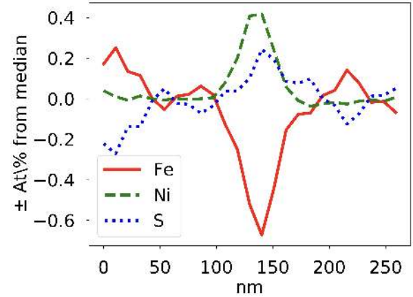
Figure 4. Average of three linescans across Ni-rich bands. The Ni content is higher and the Fe content lower in the Ni-rich bands. The variability of S across bands is not clear.
