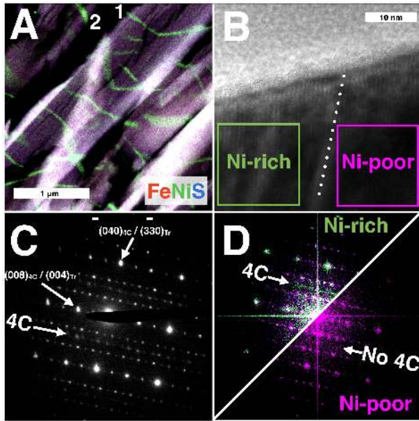
Figure 3. A) EDS map showing troilite (purple) with Ni-rich bands (green). B) HRTEM image down the [110] troilite axis with a Ni-rich band on the left and a Ni-poor region on the right. The boxes show the regions used to produce FFTs of each region (shown in D). C) SAED of region including Ni-rich and poor regions down the [110] (troilite) or [100] (pyrrhotite 4C) zone axis. Pyrrhotite 4C superlattice reflections (4C) are marked alongside troilite (Tr). D) HRTEM FFT shows the same pattern. Purple spots are from the FFT of the Ni-poor region (box shown in B) and green shows the FFT from the Ni-rich region (box shown in B). The Ni-rich FFT shows the pyrrhotite 4C superlattice reflections.
