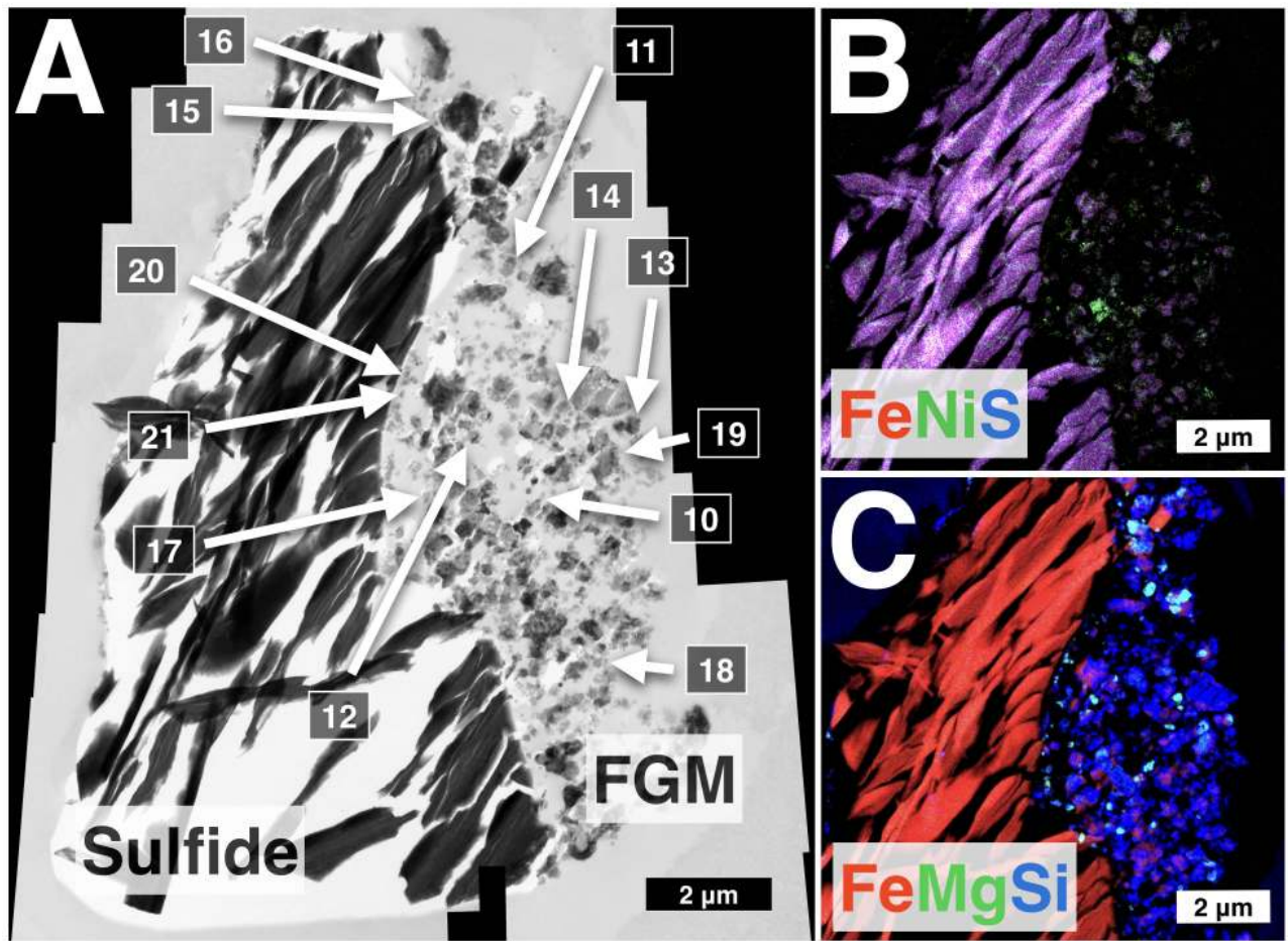
Figure 2. A) Mosaic of brightfield TEM images of Andromeda showing the sulfide on the left, and fine-grained material (FGM) on the right. Objects in the FGM are labeled according to their names in Table 2. B) EDS map of the FGM with iron (red), nickel (green), and sulfur (blue). The Ni content in the FGM is significantly higher than the Ni content of the primary sulfide impactor. C) EDS map of the FGM with iron (red), magnesium (green), and silicon (blue). Mg-rich grains include equilibrated aggregates, GEMS and altered objects. The interstitial space is filled with epoxy.
