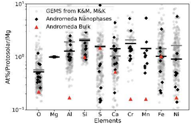
Figure 11. Comparison of thermally modified and pristine GEMS-like and EA-like objects within Andromeda's fine grained material (FGM) to GEMS from literature. Black diamonds indicate Andromeda nanophase object compositions normalized to protosolar and Mg. Horizontal black bars are the mean composition. Gray circles indicate GEMS compositions from Keller and Messenger (2011) (K&M) and Messenger et al. (2015) (M&K). Horizontal gray bars are the GEMS mean composition. Red triangles show the bulk composition of the Andromeda FGM which is distinctly not GEMS-like since it contains pyroxenes, sulfides, and other astromaterials.
