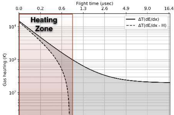
Figure 13. Vaporized gas temperature as a function of time. The top solid line shows simple heating of gases and serves as an upper limit for the temperature. The bottom dashed curve heats the gases only after accounting for the heat used to volatilize aerogel and sulfide, as well as to dissociate of \text{FeS}(\text{g}) \rightarrow \text{Fe}(\text{g}) + \text{S}(\text{g}) and \text{SiO}_2(\text{g}) \rightarrow \text{SiO}(\text{g}) + \text{O}(\text{g}) or \text{Si}(\text{g}) + \text{O}_2(\text{g}) . The bottom curve serves as a lower limit for the heating. The shaded region shows the range of possible temperatures as a function of depth per the model. The heating zone marks the region where gas temperatures exceed 1000 K and lasts for < 1 \mu\text{s} and < 3 \text{ mm} into the track.
