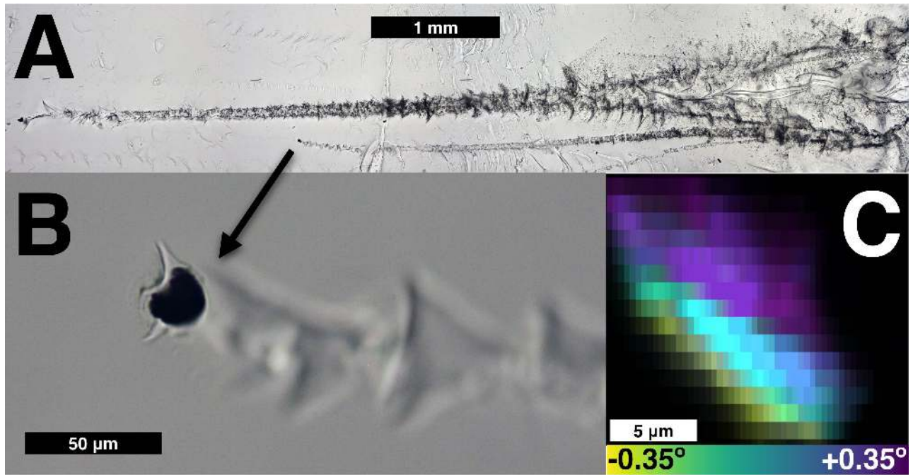
Figure 1. A) Optical mosaic image of track 191 produced from image stacks at varying focus. Andromeda was found at the end of an 8.8 mm track. The arrow connects the location of Andromeda in the track to panel B. B) Optical zoom-in of Andromeda. C) XRD topograph of Andromeda showing that the sulfide is a single crystal but with three subgrains spaced in 0.35^\circ increments. Due to sample preparation and beamline geometry panel C is not at the same viewing angle as panels A and B.
