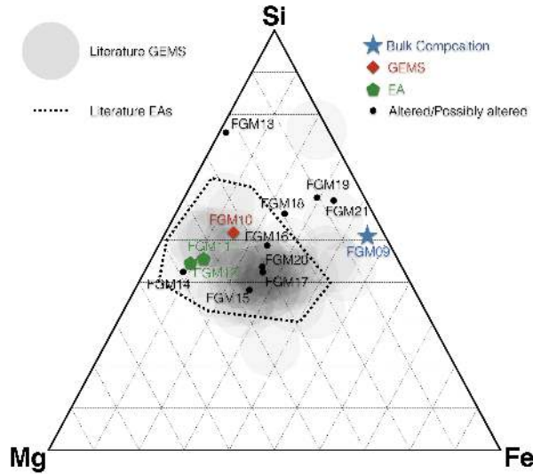
Figure 10. Ternary plot showing the compositions of fine grained materials in Andromeda compared to the GEMS field from Messenger et al. (2015), and EA field from Keller and Messenger (2009). SiO 2 enrichment from aerogel mixing would push all the points toward the Si corner. FGM09 is the bulk composition of the entire FGM region including many objects which are not GEMS or EAs.
