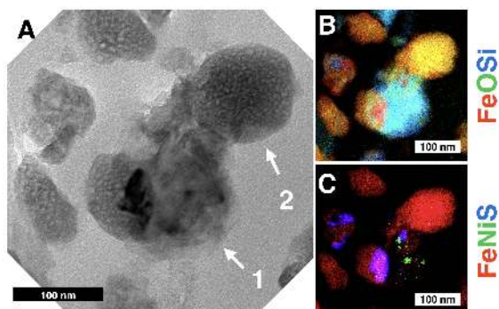
Figure 7. A) BF image of FGM16. The location marked (1) is the equilibrated aggregate. (2) is one of several Fe-oxides. B) EDS map showing the Si-rich aggregate (cyan) contrasted with the Fe-oxides (yellow). C) EDS map showing the presence of Ni-rich metals inside the equilibrated aggregate (green), the Fe-oxides (red) and sulfides (purple).
