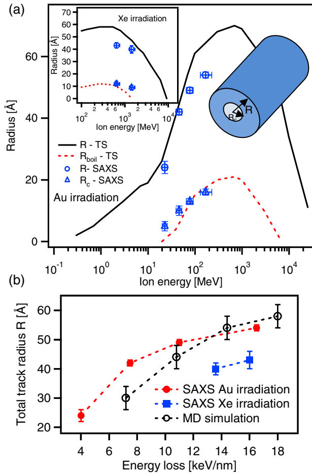
FIG. 2 (color online). (a) Calculations of molten ( R -TS) and boiling ( R_{\text{boil}} -TS) radii of Au irradiation (inset: Xe irradiation) in a -SiO 2 using an i-TS model. The symbols show measurements of total track radii (R-SAXS, circles) and core radii ( R_c -SAXS, triangles). (b) Total track radii as a function of electronic energy deposition measured by SAXS and obtained from MD simulations.
