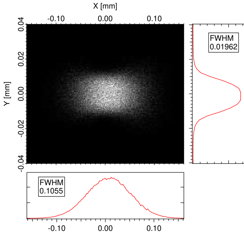
Figure 4: Spot pattern and beam intensity profiles at the sample plane at 17 eV (600 l/mm grating, c=2.25 ). The vertical exit slit opening was 50 \mu\text{m} while there was no limitation horizontally. FWHM values for the width and height show 106 \mu\text{m} and 20 \mu\text{m} , respectively. This image was obtained by simulating the solid state branch.
