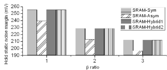
Fig. 17. The hold static noise margins of FinFET SRAM cells with different \beta ratios. T = 90\text{ }^\circ\text{C} .
