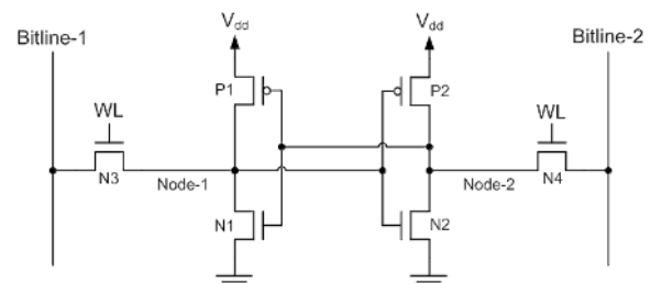
Fig. 1. A standard 6T SRAM cell.
