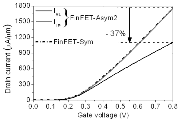
Fig. 12. Comparison of saturation region drain currents that are produced by n-type FinFET-Asym2 and FinFET-Sym for various gate voltages. V_{\text{drain}} = 0.8\text{ V} , V_{\text{source}} = 0\text{ V} , T = 25^\circ\text{C} .
