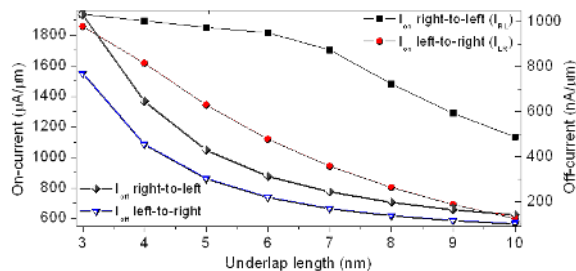
Fig. 5. Variation of the on-current and off-current of n-type asymmetric FinFET-Asym1 with the underlap length. The underlap length on the right side is varied from 3 nm to 10 nm. The overlap on the left side is 1.5 nm. T = 25^\circ\text{C} .
