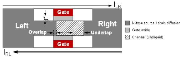
Fig. 4. Cross-sectional view (along the gate length) of an asymmetric n-type FinFET-Asym1.
