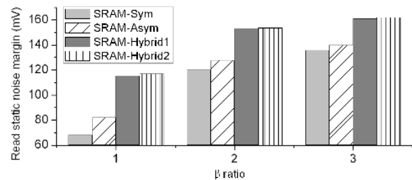
Fig. 16. The read static noise margins of FinFET SRAM cells with different \beta ratios. T = 90\text{ }^\circ\text{C} .
