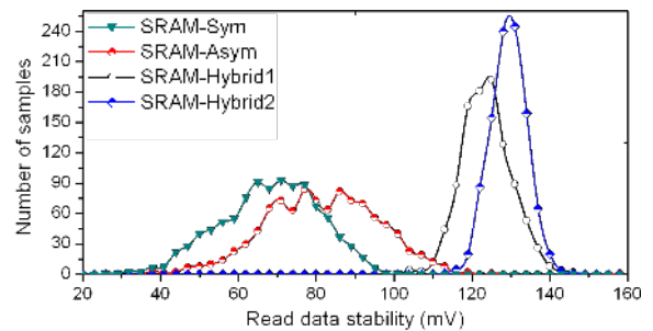
Fig. 25. Statistical read static noise margin distributions of FinFET SRAM cells. \beta = 1 . T = 90^\circ\text{C} .
