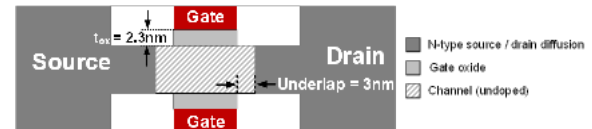
Fig. 2. Cross-sectional view (along the gate length) of n-type FinFET with symmetric gate-underlaps (FinFET-Sym). Gate work-function = 4.46 eV. Fin height = 15 nm.
