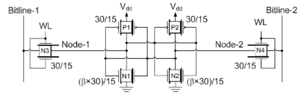
Fig. 14. The second new hybrid FinFET SRAM cell (SRAM-Hybrid2) with asymmetrically gate-underlapped bitline access transistors. FinFET-Asym2s are represented with asymmetrical thick lines along the channel. The transistors in cross-coupled inverters are symmetrical FinFETs (See Fig. 2 for the FinFET-Sym profile). The transistor sizes (width/length) are in nanometers assuming a 15 nm FinFET technology.
