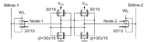
Fig. 9. A new hybrid six-FinFET SRAM cell with asymmetrical bitline access transistors (SRAM-Hybrid1). The bitline access transistors are asymmetrically overlapped / underlapped FinFETs (see Fig. 6 for the FinFET-Asym1 profile). The transistors in cross-coupled inverters are symmetric FinFETs. The transistor sizes (width/length) are in nanometers assuming a 15 nm FinFET technology.
