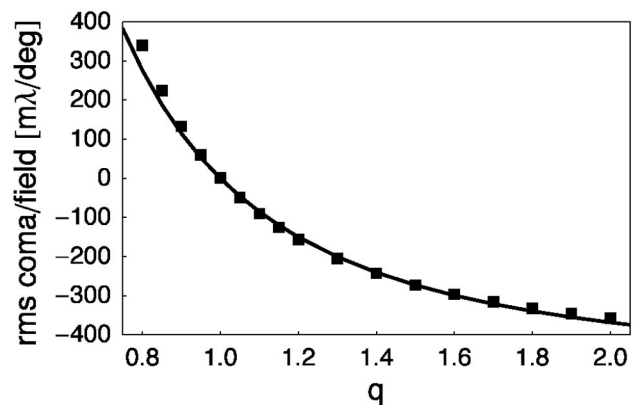
Fig. 5. Sensitivity of coma for field use of the lens as a function of the q parameter that interpolates between the Abbe and the Herschel conditions (squares) and a fit proportional to 1 - q^{-2} (solid curve).
