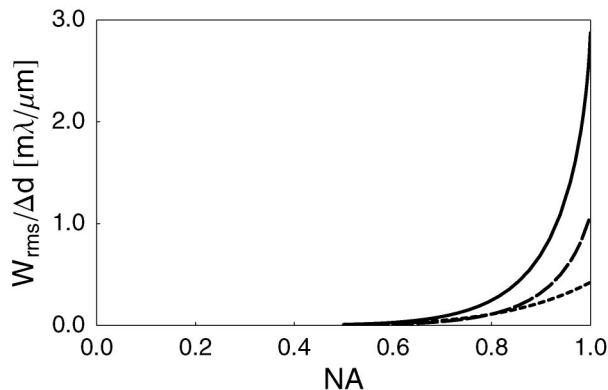
Fig. 2. Residual aberration sensitivity as a function of NA (solid curve) and approximation by the single Zernike term A_{60} (long-dashed curve) and by the Seidel term proportional to NA^6 (short-dashed curve).
