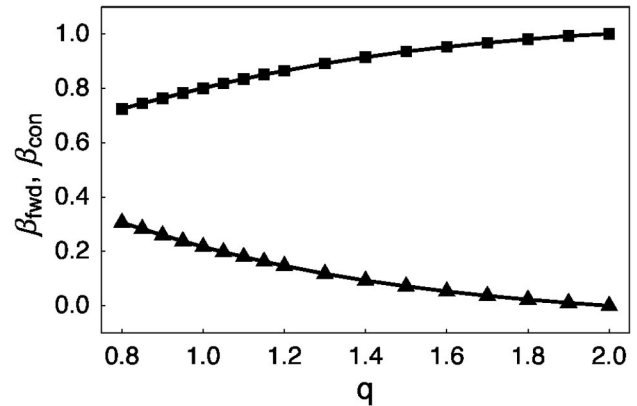
Fig. 4. Numerically determined parameters \beta_{\text{con}} (squares) and \beta_{\text{fwd}} (triangles) for a lens with 0.85 NA as a function of the q parameter that interpolates between the Abbe and the Herschel conditions.
