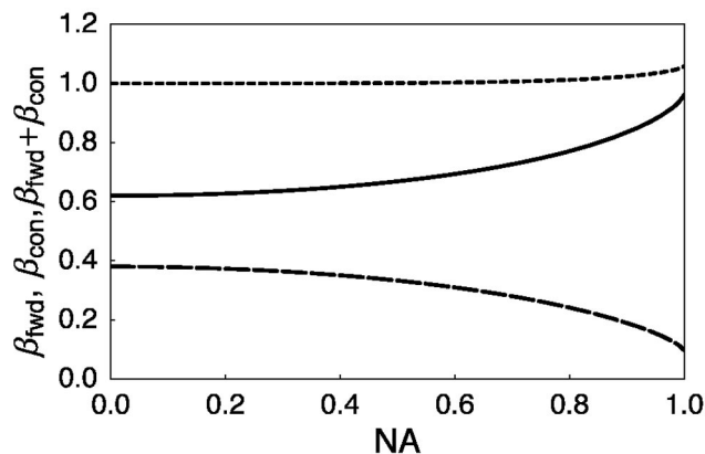
Fig. 3. Parameter \beta_{\text{con}} that describes the relative change of conjugate (solid curve), the parameter \beta_{\text{fwd}} that describes the relative change in free working distance (long-dashed curve), and the sum of the two parameters \beta_{\text{con}} + \beta_{\text{fwd}} (short-dashed curve) as a function of NA.
