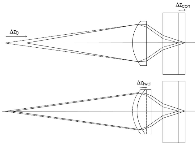
Fig. 1. Changing the axial focal position can be achieved by changing the conjugate of the objective lens (top) or by changing the free working distance (bottom).
