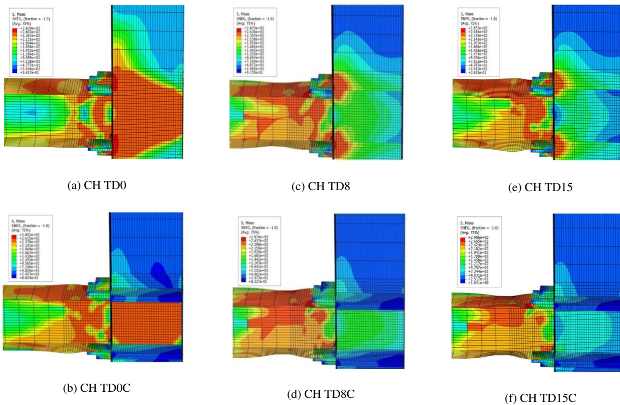
Fig. 11: Von Mises stress contours (MPa) of channel connection in the connection region for different panel zones at the end of the cyclic loading
