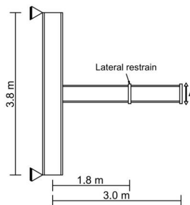
Fig. 3: Geometry and condition of supports
