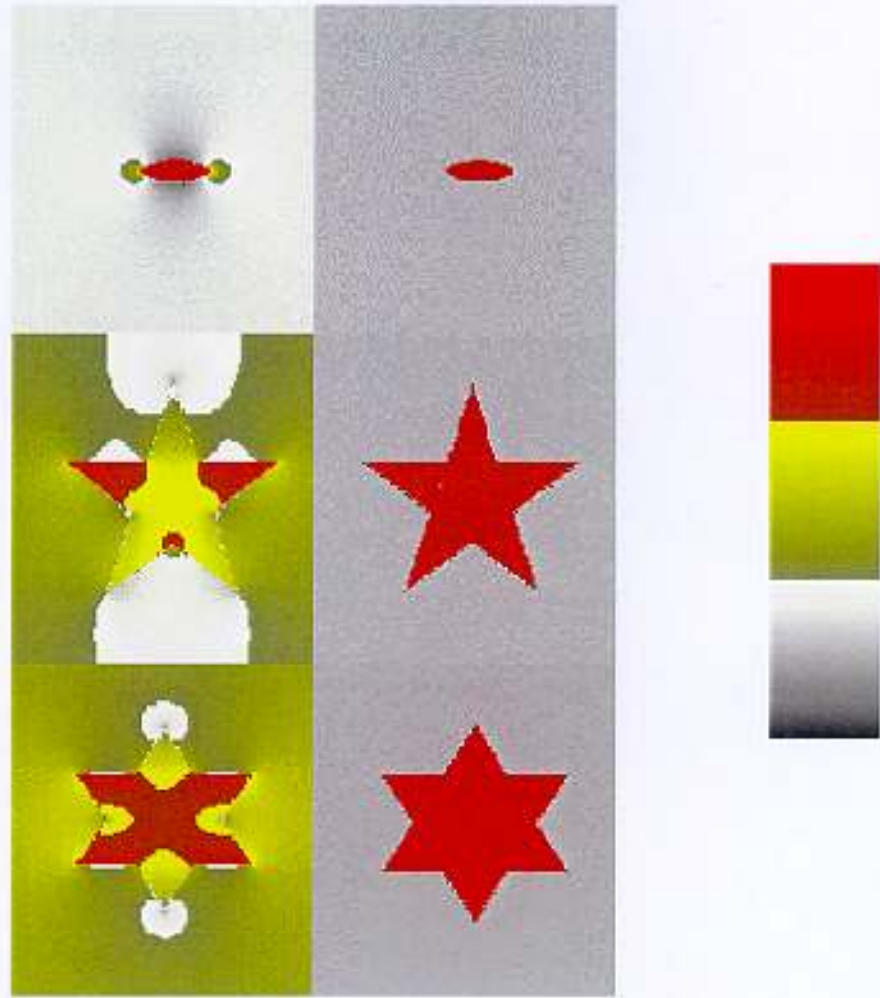
Figure 11: Thermal stress for inclusions with the same elastic moduli as the matrix, but different thermal eigenstrain. Stress is high (top) to low (bottom) in color bar. Left: -\sigma_{xx} , right: negative of the trace of the stress tensor. Images from top: Ellipse, 5-pointed star, 6-pointed star.
