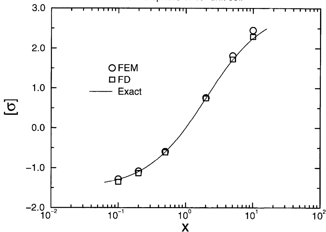
Figure 8: Intrinsic conductivity for a 15 pixel diameter sphere embedded in a 40^3 unit cell, as a function of the ratio of the sphere conductivity to the matrix conductivity. Finite element and finite difference data and the exact result are compared.
