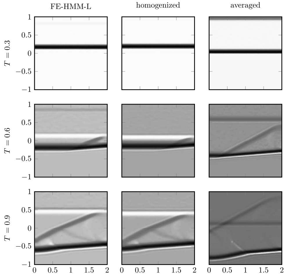
FIG. 7. Two-dimensional layered topography. Snapshots of the FE-HMM-L solution u_H (left), the solution u^0 of the homogenized equation (2.5) (middle), and that with a locally averaged tensor (right) are shown at times T = 0.3, 0.6, 0.9 .
