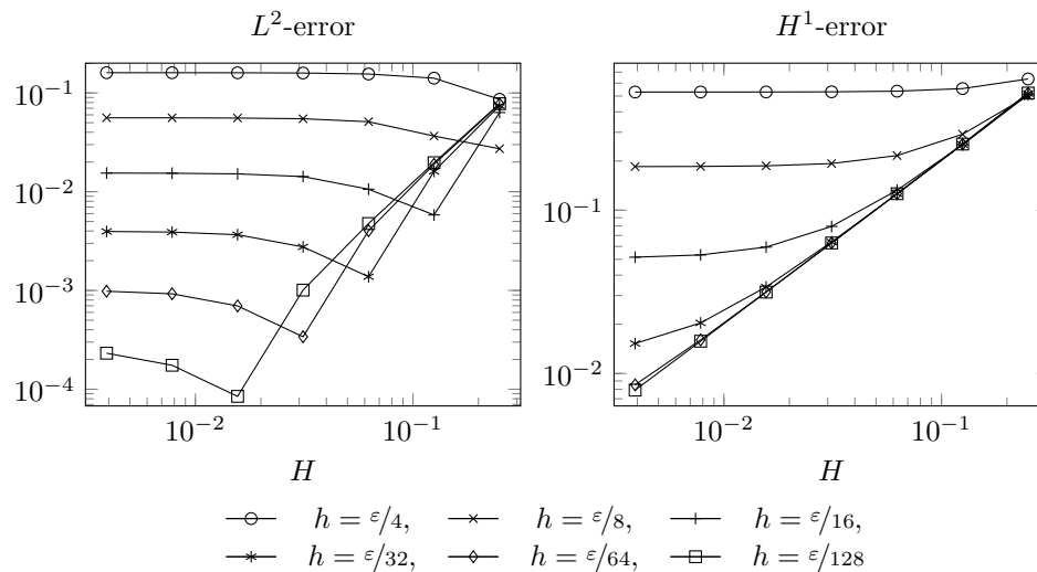
FIG. 2. One-dimensional periodic medium. L^2 -error (left) and H^1 -error (right) \|u_H - u^0\| at time T = 2.75 , where only the macro mesh size H is refined, but the micro mesh size h is kept fixed. The different lines correspond to different values of h .
