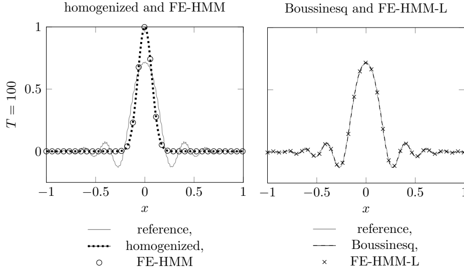
FIG. 8. One-dimensional periodic medium. Left: The true solution u^\epsilon , the solution u^0 of (2.5), and the FE-HMM scheme from [8] are shown at T = 100 . Right: The true solution u^\epsilon , the solution u^{\text{eff}} of the Boussinesq equation (1.3), and the FE-HMM-L solution u_H all coincide at T = 100 .
