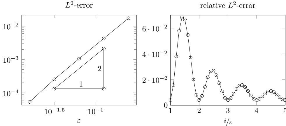
FIG. 3. One-dimensional periodic medium. Error \|u_H - u^0\| at time T = 2.75 . Left: L^2 -error versus the period \epsilon . Right: Relative L^2 -error versus the ratio between \delta and \epsilon .
