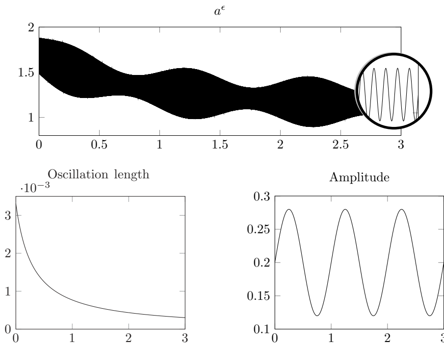
FIG. 4. One-dimensional nonperiodic medium. Top: Multiscale tensor a^\epsilon(x) for \epsilon = 1/500 with a zoom at x = 3 . Bottom: Change of the period (left) and the amplitude (right).
