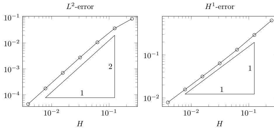
FIG. 1. One-dimensional periodic medium. L^2 -error (left) and H^1 -error (right) \|u_H - u^0\| at time T = 2.75 , with simultaneous refinement of the macro mesh size H and the micro mesh size h .
