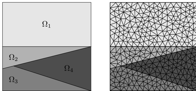
FIG. 6. Two-dimensional layered topography. Left: The computational domain \Omega with its subdomains. Right: A sample triangulation of \Omega which respects the inner interfaces.
