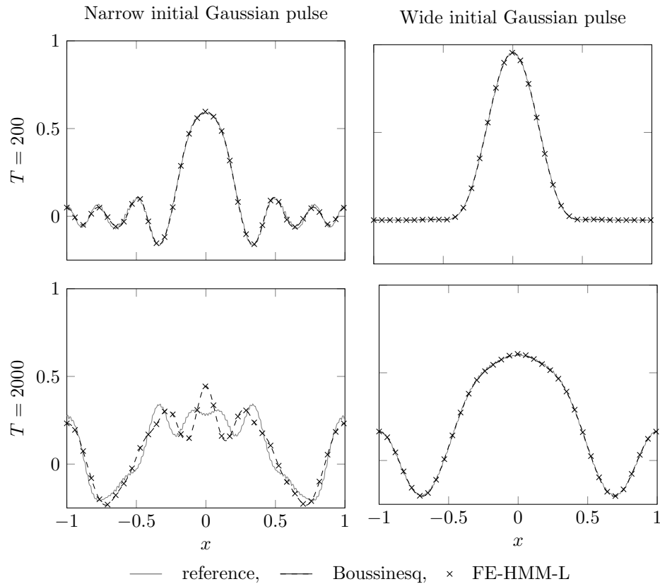
FIG. 9. One-dimensional periodic medium. The solutions u^\varepsilon , u^{\text{eff}} , and u_H are shown for two different initial conditions at T = 200 (top) and T = 2000 (bottom). Left: Narrow initial Gaussian pulse ( \sigma^2 = 1/100 ). Right: Wide initial Gaussian pulse ( \sigma^2 = 1/20 ). In the lower left frame u^{\text{eff}} and u_H coincide, yet both differ from u^\varepsilon .
