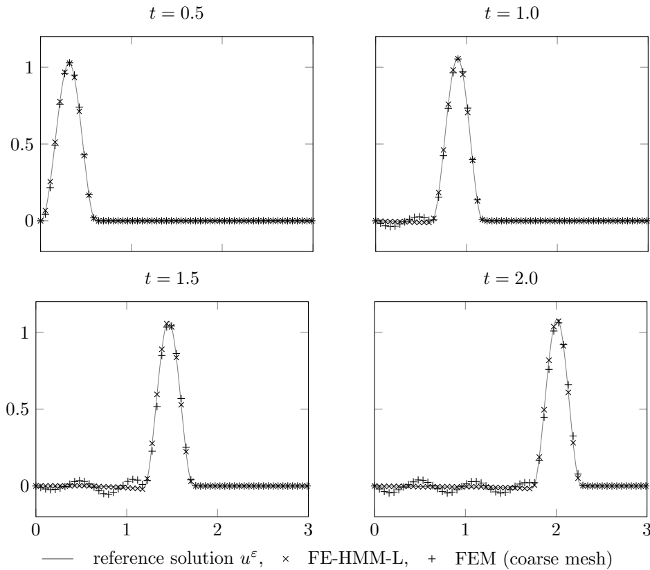
FIG. 5. One-dimensional nonperiodic medium. Snapshots of the reference, the FE-HMM-L, and the FEM solution on a coarse mesh at times T = 0.5, 1.0, 1.5, 2.0 . The (unresolved) FEM solution deviates from the (true) fully resolved reference solution, whereas the FE-HMM-L, computed on the same coarse mesh, approximates well its macroscopic behavior.
