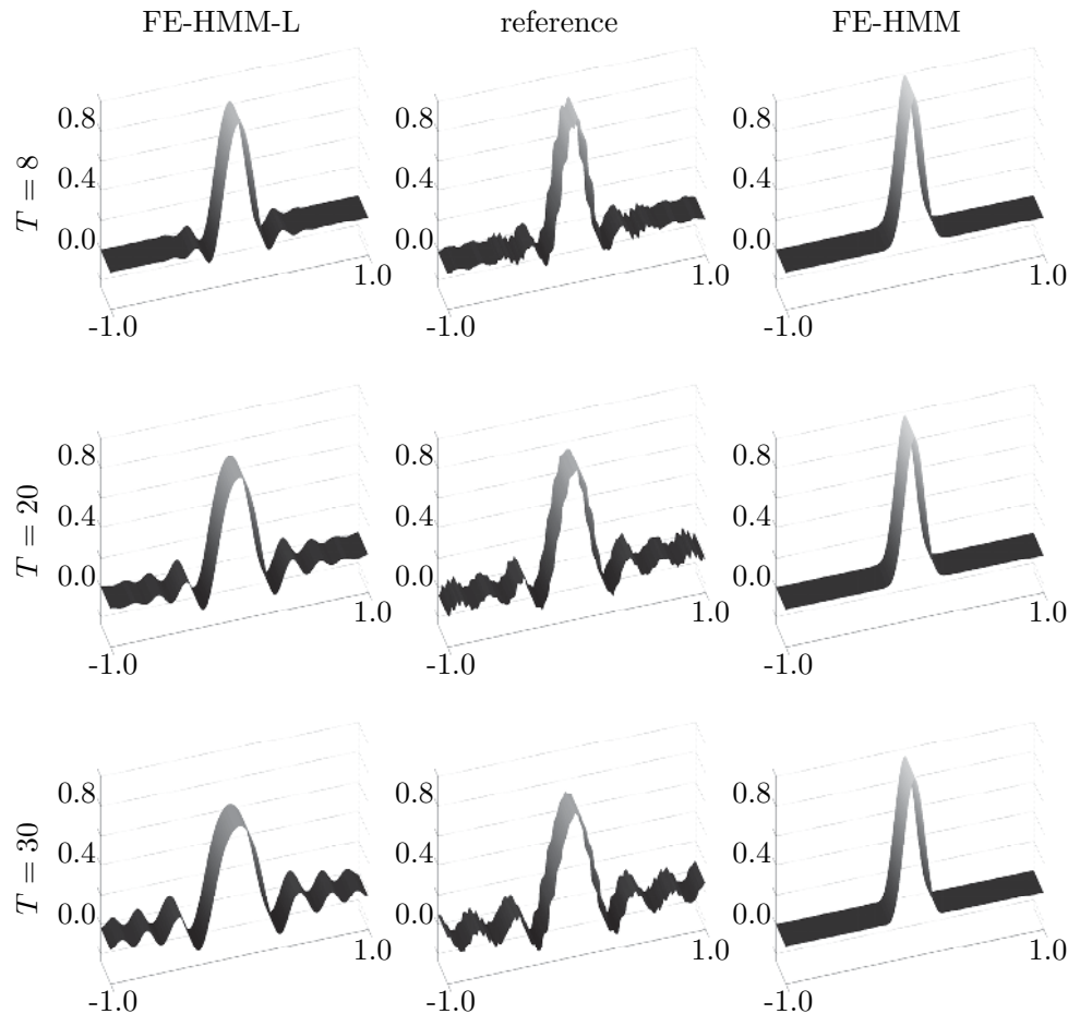
FIG. 10. Two-dimensional wave guide. Snapshots of the FE-HMM-L u_H (left), the reference u^\varepsilon (middle), and the FE-HMM (right) solutions at times T = 8, 20, 30 . The physical dispersive effects are correctly captured by the FE-HMM-L but not by the FE-HMM scheme.
