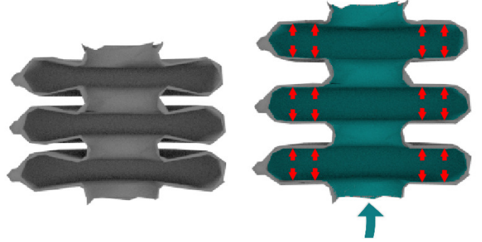
Fig. 3: Pressure actuation
