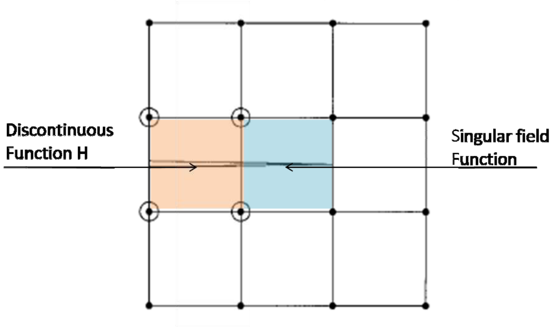
Figure 11 Enriched element around crack tip
