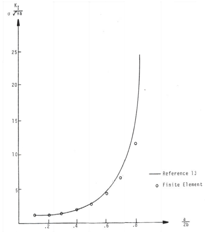
Figure 7 Stress Intensity Factor
