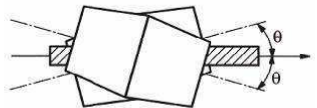
Fig. 2: Orientation of the rolls with respect to the billet [1]
