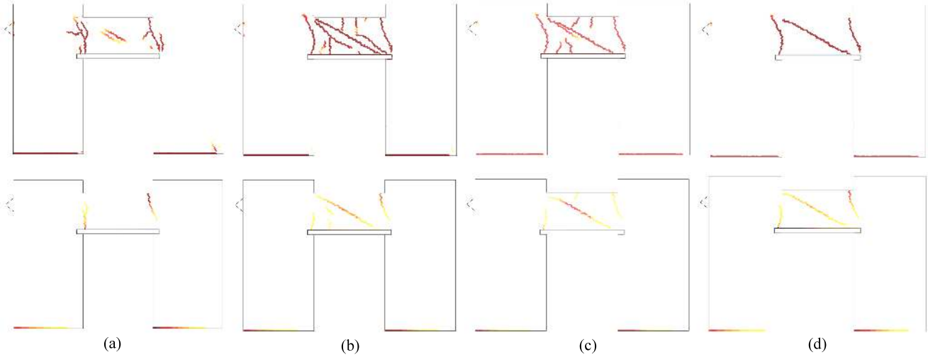
Fig. 17: Contour of tensile damage (left) and maximum principal strain (right): (a) r_{excl} = 0.1 m , (b) r_{excl} = 0.2 m , (c) r_{excl} = 0.3 m , (d) r_{excl} = 0.5 m (horizontal displacement d = 0.21 m ).
