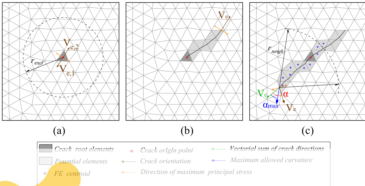
Fig. 2: Simulation of internal cracking with the crack-tracking technique: (a) internal crack root element with the two opposite vectors of the crack propagation, (b) labelling of the next potential elements towards the first side of the crack, (c) labelling of the next potential elements towards the second side of the crack and use of the maximum curvature criterion .
