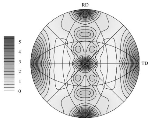
Figure 10. Approximation of the experimental (100) pole figure.
