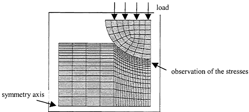
Fig. 7 : two-dimensional model
