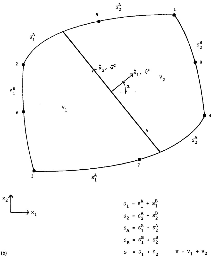
Figure 2. Finite element with embedded localization line: (a) 1D element; (b) 2D element
