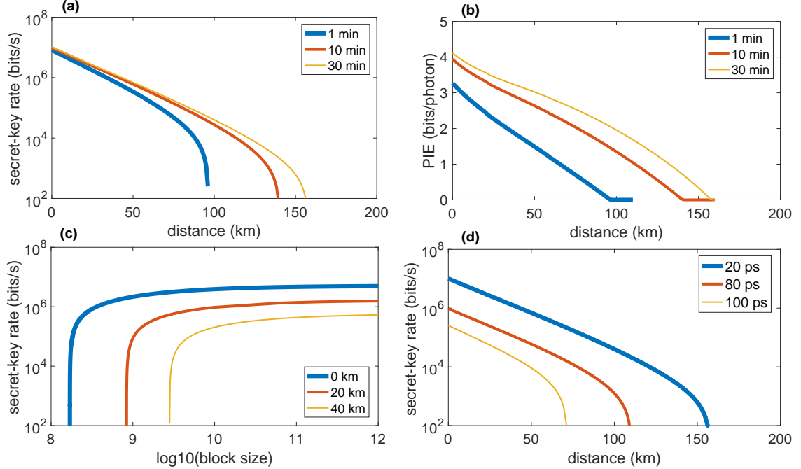
FIG. 1: Numerically-evaluated performance of time-energy HD-QKD with threshold code distance d_0 = 2 and other parameters as listed in Table I. (a) Secret-key rate (bits/s) versus transmission distance (km) for different total running times of transmission: top curve (yellow) 30 min, middle curve (red) 10 min, bottom curve (blue) 1 min. (b) PIE (bits/photon) versus transmission distance (km) for different running times: top curve (yellow) 30 min, middle curve (red) 10 min, bottom curve (blue) 1 min. (c) Secret-key rate (bits/s) versus block size (running time/clock rate) for different transmission distances: top curve (blue) 0 km, middle curve (red) 20 km, bottom curve (yellow) 40 km. (d) Secret-key rate (bits/s) versus transmission distance (km) for different time-bin durations \delta , where the running time is fixed at 30 min: top curve (blue) 20 ps, middle curve (red), 80 ps, bottom curve (yellow) 100 ps.
