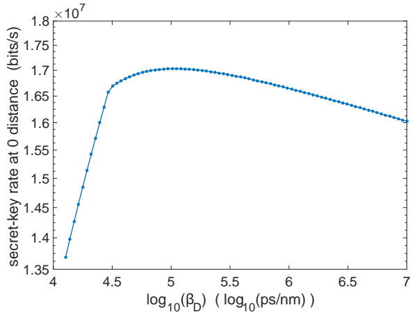
FIG. 2: Secret-key rate at zero distance versus GVD coefficient \log_{10}(\beta_D) for 30 min running time. The conventional units for \beta_D are employed here: ps per nm of bandwidth at telecom wavelength. The secret-key rate at zero distance achieves its 17 Mbit/s maximum at \beta_D = 10^5 ps/nm at telecom wavelength, which is equivalent to 2 \times 10^6 ps 2 in the units used in Table I.
