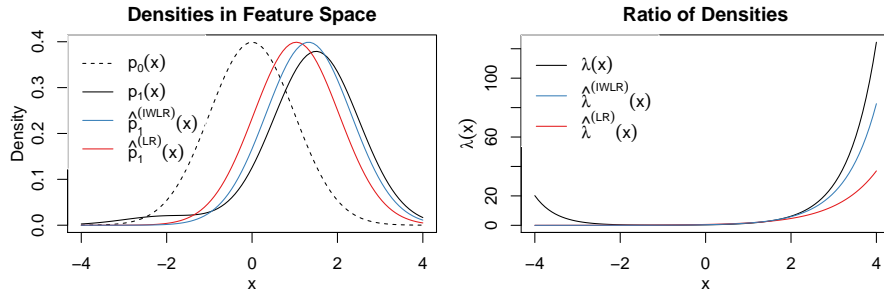
FIG 4. Large-sample estimates for the simulation study, misspecified case. The black curves represent the true presence density (left panel) and intensity (right panel). The blue and red curves show the fitted densities using IWLR and standard logistic regression with n_0 = n_1 .
