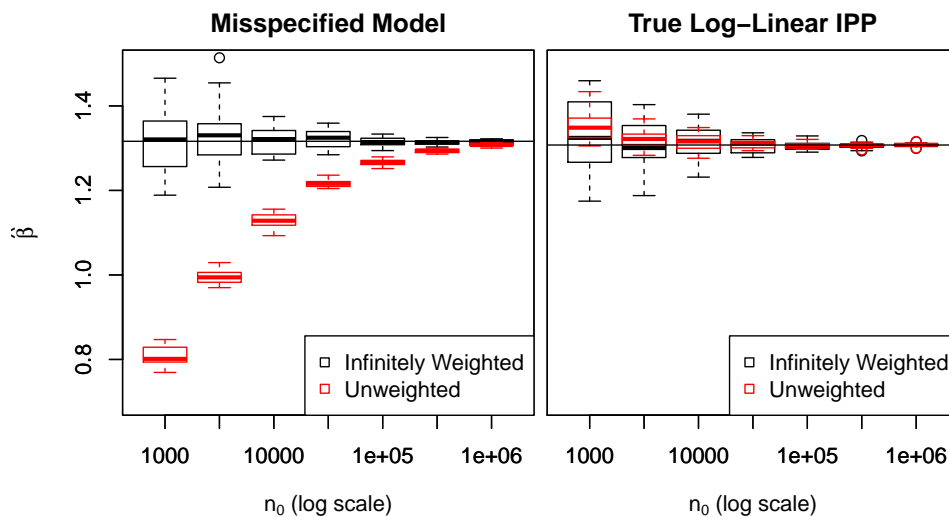
FIG 5. \hat{\beta} estimates for simulation study with n_1 = 3000 and varying n_0 . Unweighted logistic regression may require a very large background sample before convergence when the model is misspecified.
