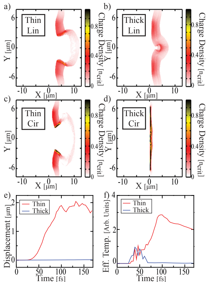
FIG. 4: (Color online) Proton density space of OSIRIS 2D PIC simulations for a) thin linear, b) thick linear, c) thin circular, and d) thick circular cases taken at 168 fs. For the circular case, the mean target displacement along the laser axis v. time is shown in e), and the effective temperature v. time is shown in f). “Thin” and “thick” correspond to a total target thickness of 36 nm and 108 nm respectively with the target left justified at an x position of 0.
