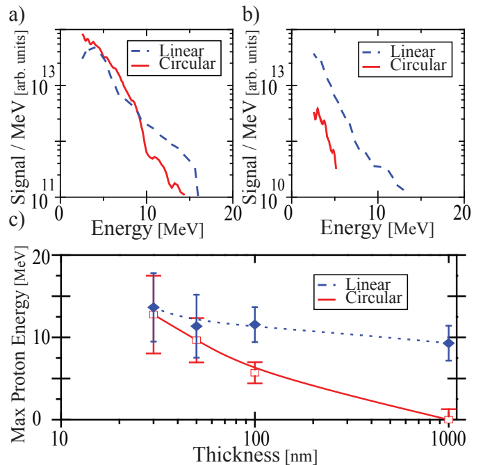
FIG. 1: (Color online) Proton energy spectra for both right-hand circular and linearly polarized laser pulse interactions for a) 30 nm and b) 100 nm thickness SiN targets. Maximum proton energy vs. target thickness is also shown (c) with lines shown as visual aid only.
