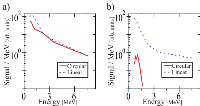
FIG. 2: (Color online) Electron energy spectra for right-hand circular (solid) and linear (dashed) polarized laser pulse interaction for a) 30 nm and b) 100 nm SiN targets.
