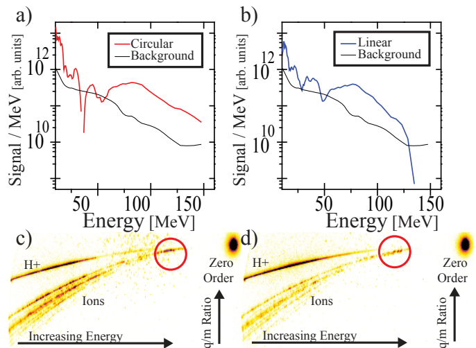
FIG. 3: (Color online) C_6^+ energy spectra for a) right-hand circular and b) linear polarized laser pulse interaction for 30 nm SiN targets. Detector background levels are shown for comparison. Raw spectra are shown for c) circular and d) linear polarization, with the high energy carbon peak denoted by the red circle.
