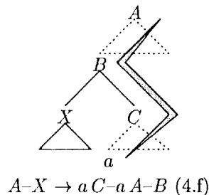
Figure 2: The highly distinctive ‘zig-zag’ or ‘lightning bolt’ configuration of nodes in the analysis tree characteristic of the use of production schema (4.f) in transform \mathcal{LC}_4 . This is the only configuration which causes an increase in stack depth in a top-down parser using a grammar transformed with \mathcal{LC}_4 .
