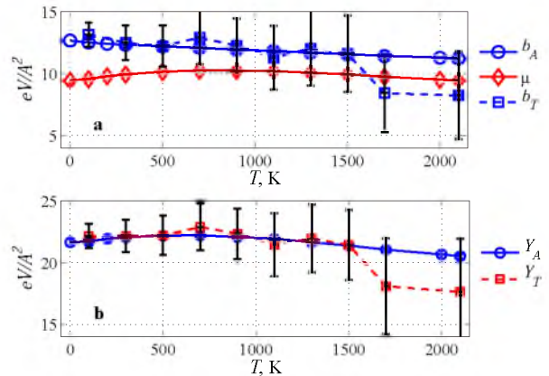
FIG. 3: a) (color online) 2D elastic moduli of graphene as of function of temperature: adiabatic bulk modulus b_A (solid blue line with circles), isothermal bulk modulus b_T (dashed blue line with squares) and shear modulus \mu (solid red line with diamonds). b) Adiabatic Young's modulus Y_A (solid blue line with circles) and isothermal Y_T (dashed red line with squares).
