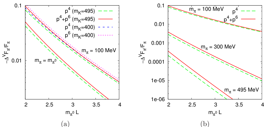
Figure 11. The finite volume corrections to the pion decay constant for a number of cases listed in table 1. Plotted is the quantity -(F_\pi^V - F_\pi)/F_\pi . (a) Physical case and (m_\pi, m_K) = (100, 495) and (100, 400) MeV. (b) m_K = 495 MeV and m_\pi = 100, 300, 495 MeV. The size L is given in units of the physical \pi^0 mass.
