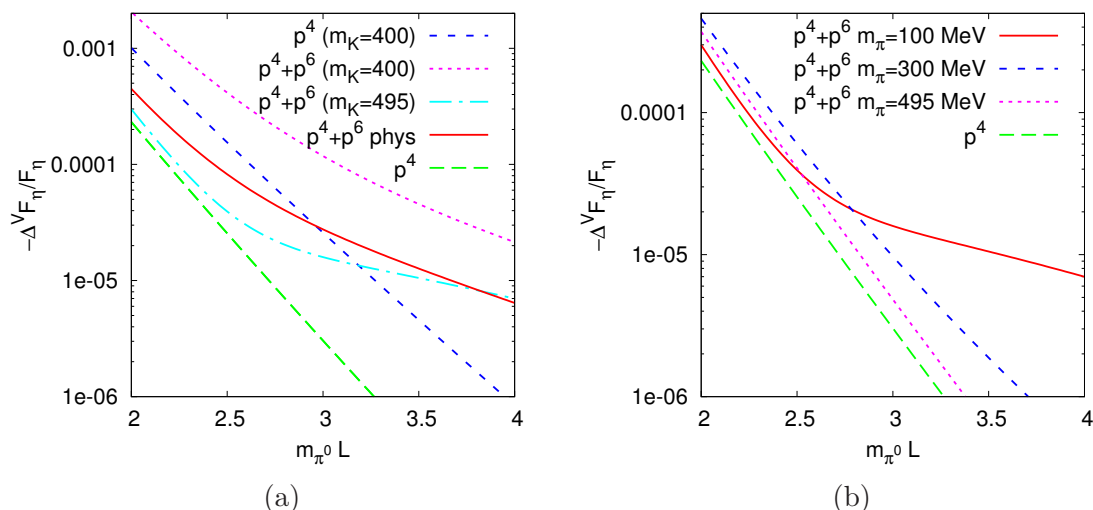
Figure 13. The finite volume corrections to the eta decay constant for a number of cases listed in table 1. Plotted is the quantity -(F_{\eta}^V - F_{\eta})/F_{\eta} . (a) Physical case and (m_{\pi}, m_K) = (100, 495) and (100, 400) MeV. The bottom line is the one-loop result for the physical case and (m_{\pi}, m_K) = (100, 495) . Others as labeled. (b) m_K = 495 MeV and m_{\pi} = 100, 300, 495 MeV. The size L is given in units of the physical \pi^0 mass.
