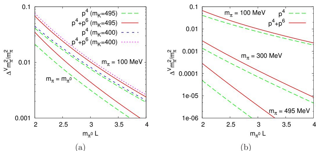
Figure 6. The finite volume corrections to the pion mass squared for a number of cases listed in table 1. Plotted is the quantity (m_\pi^{V^2} - m_\pi^2)/m_\pi^2 . (a) Physical case, bottom two lines, (m_\pi, m_K) = (100, 495) and (100, 400) MeV. (b) m_K = 495 MeV and m_\pi = 100, 300, 495 MeV. The size L is given in units of the physical \pi^0 mass.
