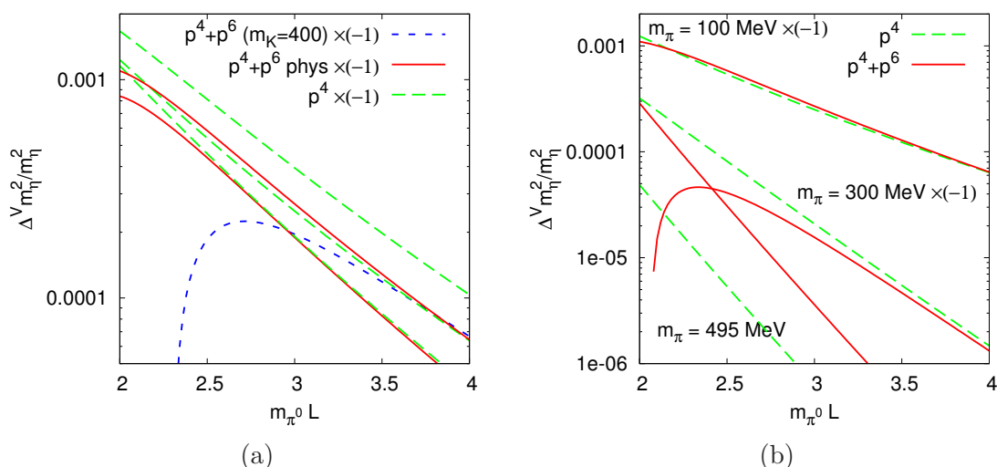
Figure 8. The finite volume corrections to the eta mass squared for a number of cases listed in table 1. for the physical case. Plotted is the quantity (m_\eta^{V2} - m_\eta^2) / m_\eta^2 . (a) Physical case and (m_\pi, m_K) = (100, 495) and (100, 400) MeV. Lines are for the one-loop result at the right bottom physical case, middle (m_\pi, m_K) = (100, 495) , top (m_\pi, m_K) = (100, 400) . The first two have only a small change due to p^6 , while for the last case there is a large cancellation between one and two-loops. (b) m_K = 495 MeV and m_\pi = 100, 300, 495 MeV. The size L is given in units of the physical \pi^0 mass.
