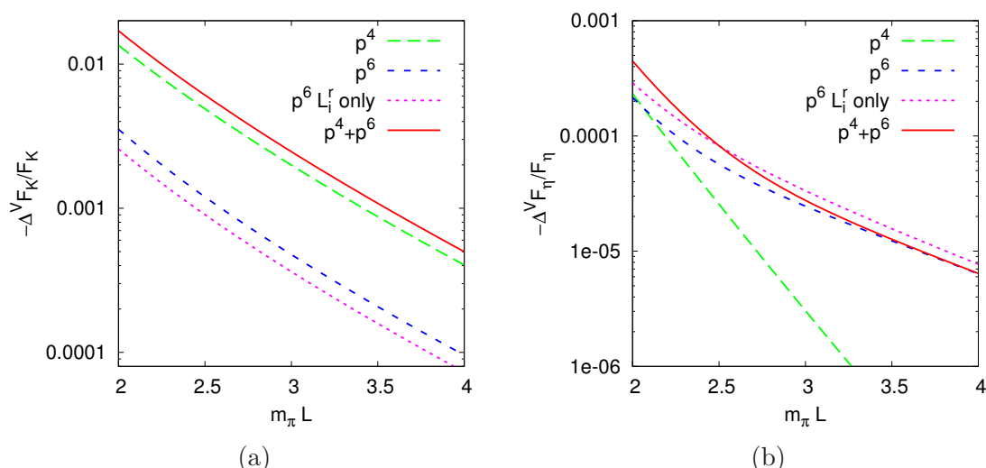
Figure 10. The corrections to the kaon and eta decay constant for the physical case. Plotted is the quantity -(F_i^V - F_i)/F_i for i = K, \eta . Shown are the one-loop, the two-loop, the sum and the two-loop L_i^r dependent part. (a) Kaon. (b) Eta.
