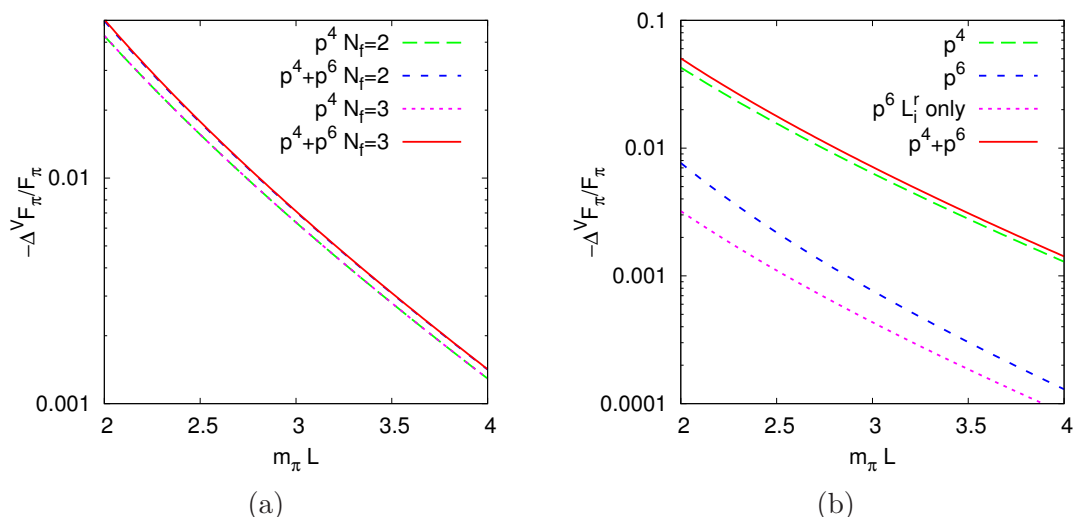
Figure 9. The finite volume corrections to the pion decay constant at m_\pi = m_{\pi^0} . All other inputs are given in the text. Plotted is the quantity -(F_\pi^V - F_\pi)/F_\pi . (a) Comparison of the two- and three-flavour ChPT results. (b) The corrections for the three-flavour case also showing the L_i^r dependent part.
