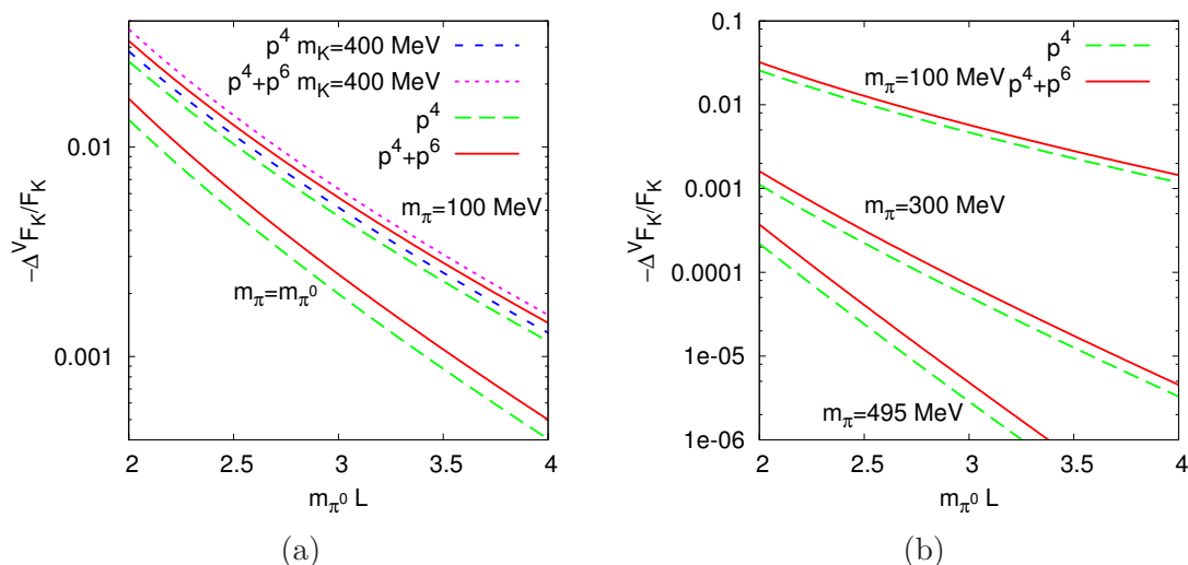
Figure 12. The finite volume corrections to the kaon decay constant for a number of cases listed in table 1. Plotted is the quantity -(F_K^V - F_K)/F_K . (a) Physical case and (m_\pi, m_K) = (100, 495) and (100, 400) MeV. (b) m_K = 495 MeV and m_\pi = 100, 300, 495 MeV. The size L is given in units of the physical \pi^0 mass.
