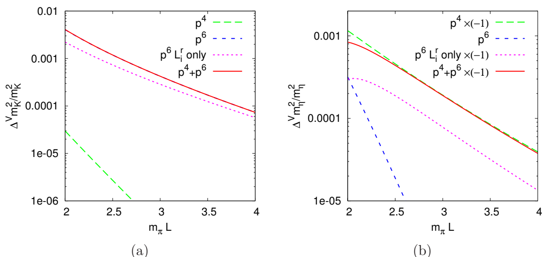
Figure 5. The corrections to the kaon and eta mass squared for the physical case. Plotted is the quantity (m_i^{V^2} - m_i^2)/m_i^2 for i = K, \eta . Shown are the one-loop, the two-loop, the sum and the two-loop L_i^r dependent part. (a) Kaon, the p^4 is so small that p^6 and p^4 + p^6 are indistinguishable. (b) Eta, note the signs, some parts are negative.
