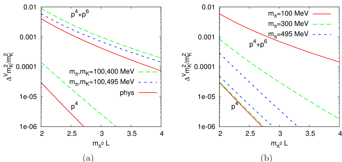
Figure 7. The finite volume corrections to the kaon mass squared for a number of cases listed in table 1. for the physical case. Plotted is the quantity (m_K^{V2} - m_K^2)/m_K^2 . (a) Physical case and (m_\pi, m_K) = (100, 495) and (100, 400) MeV. (b) m_K = 495 MeV and m_\pi = 100, 300, 495 MeV. The size L is given in units of the physical \pi^0 mass.
