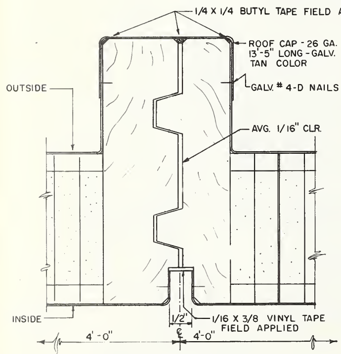
TYPICAL ROOF JOINT
