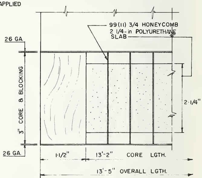
SECTION X-X TYP. SEC. AT PANEL ENDS
