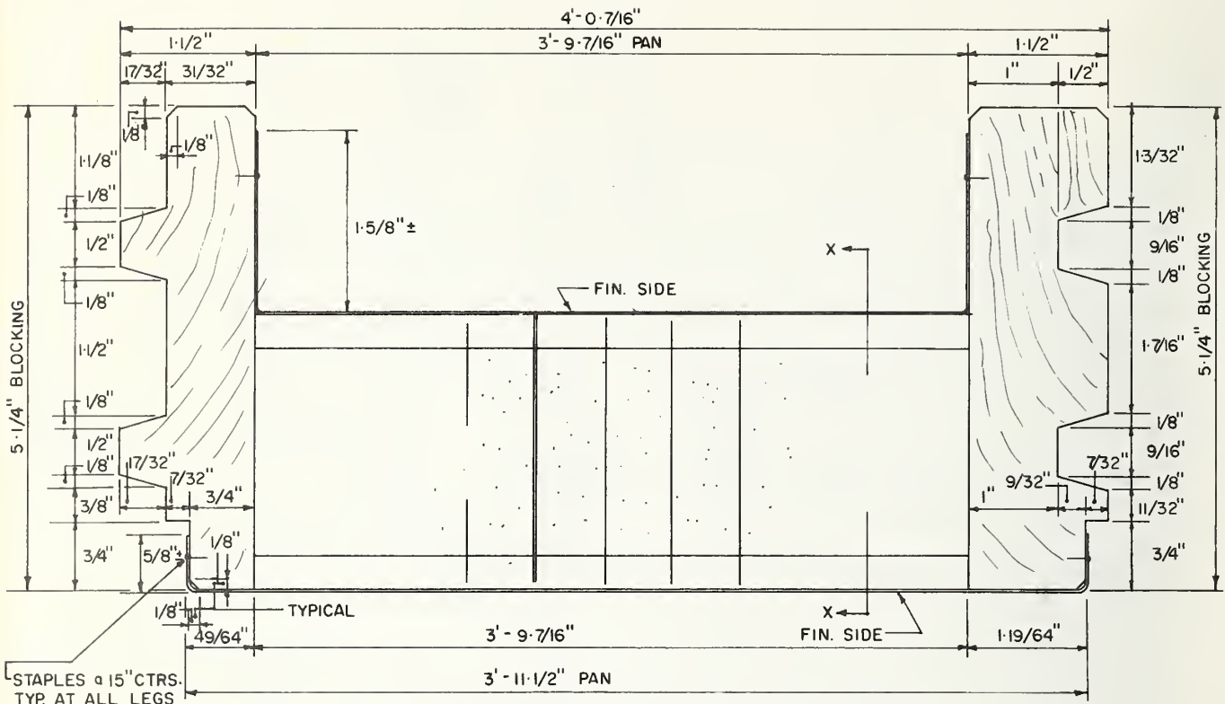
TYPICAL HORIZONTAL ROOF PANEL SECTION
