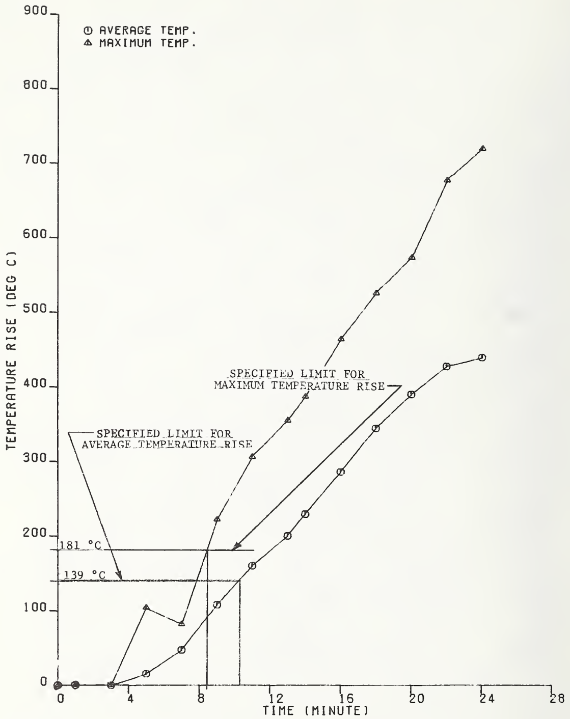
Figure 6. MAXIMUM AND AVERAGE SURFACE TEMPERATURE Roof/Ceiling Assembly
